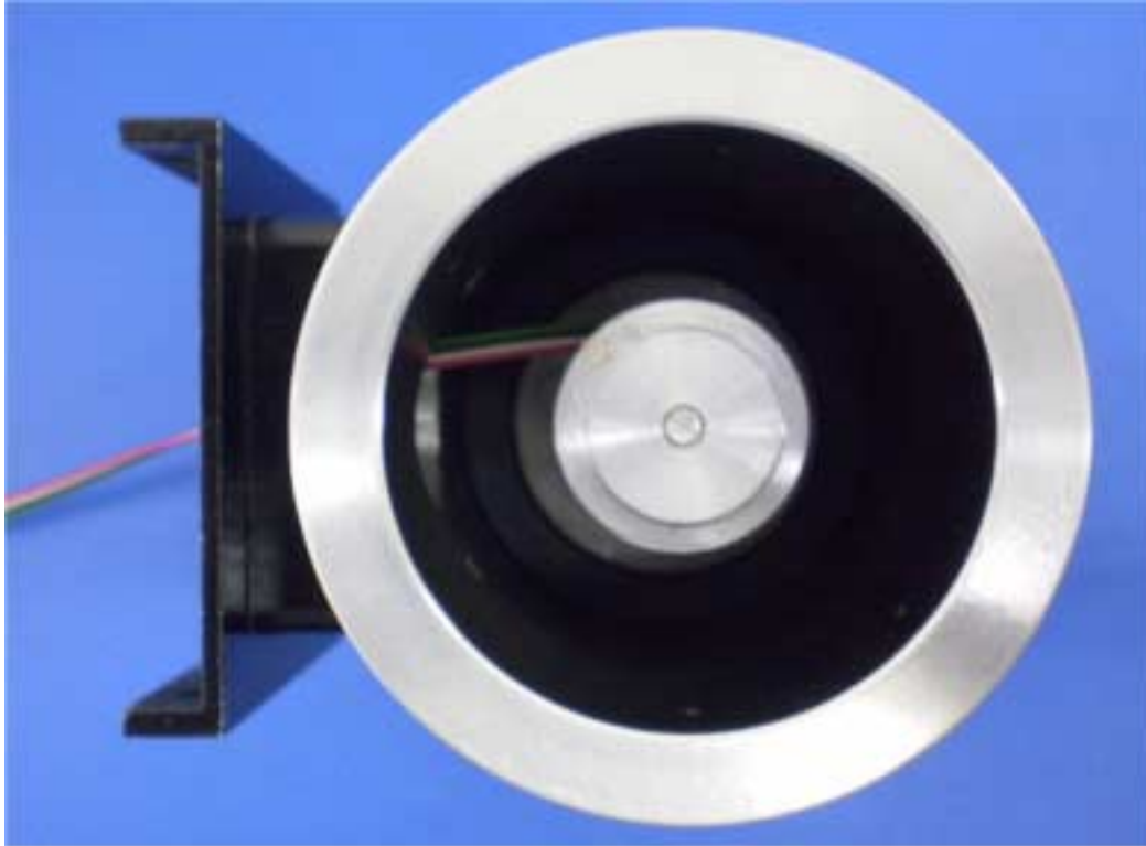
Photograph No.5 Wireless load cell top view without cover
