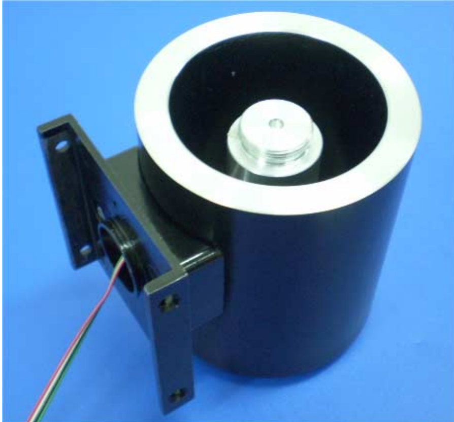
Photograph No.4 Wireless load cell without transmitter and cover
