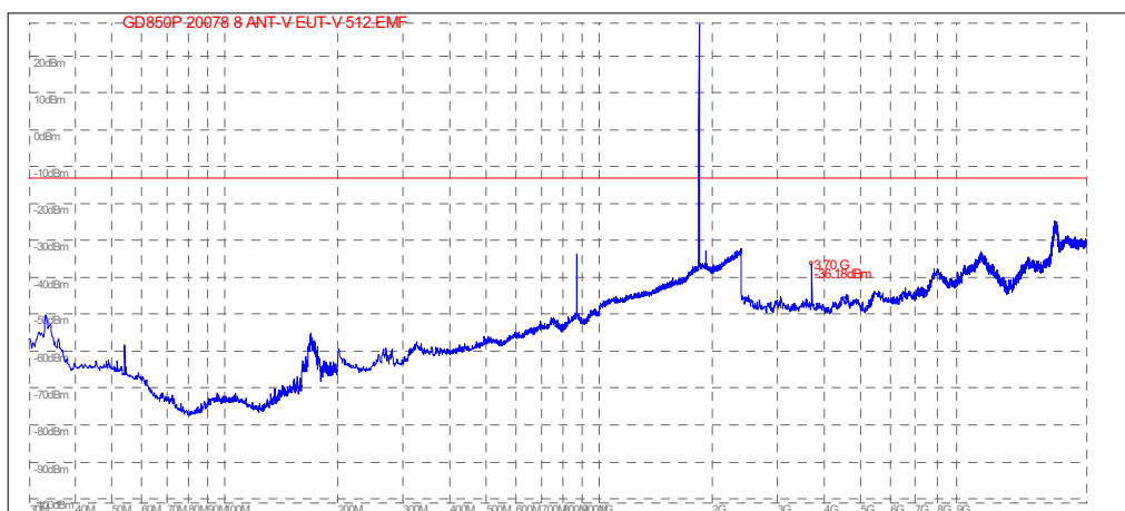
(Plot A.2: Channel = 512, Test Antenna Vertical)
