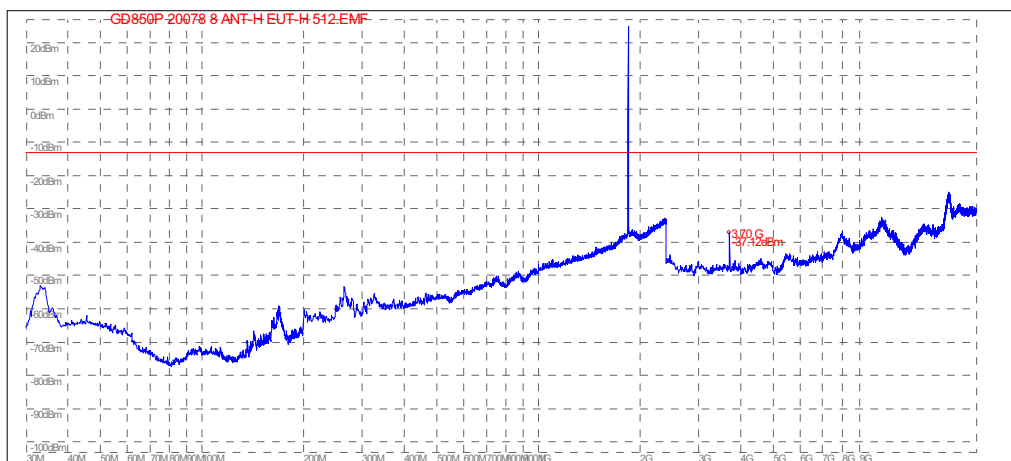
(Plot A.1: Channel = 512, Test Antenna Horizontal)
