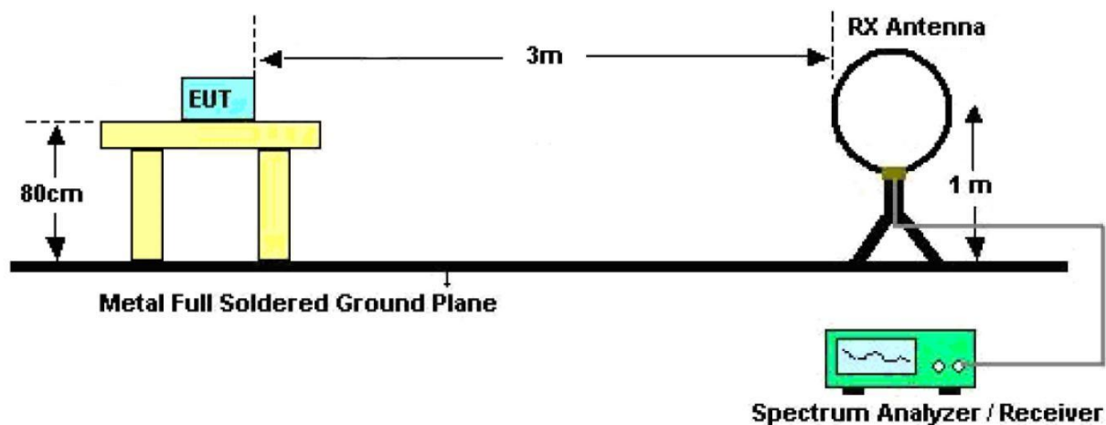
Figure 1. Below 30MHz
