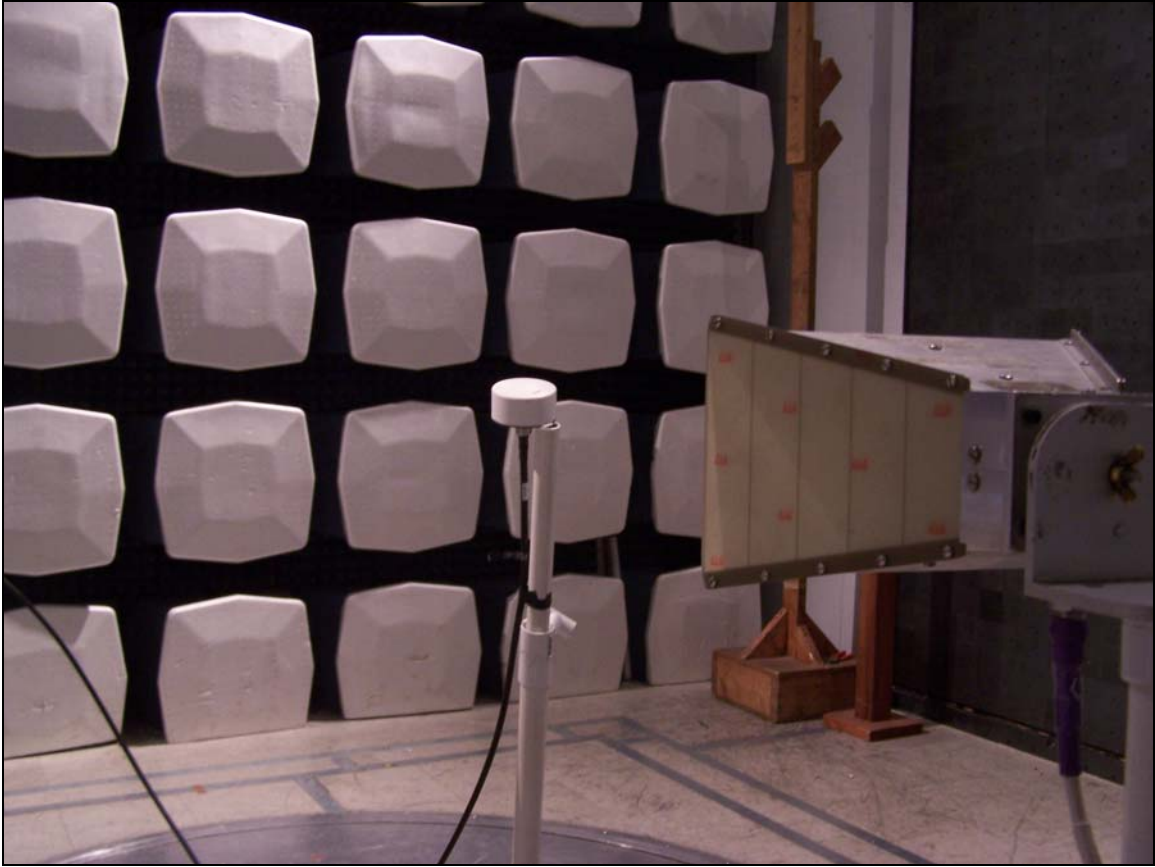
Photograph 1. Band Edge Test Setup
