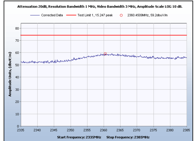
Restricted Band, 2360 MHz, Peak
