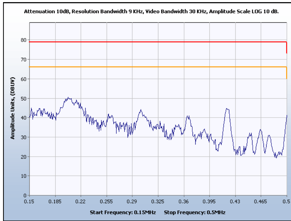
Phase Line Plot, 0.15 MHz to 0.5 MHz
