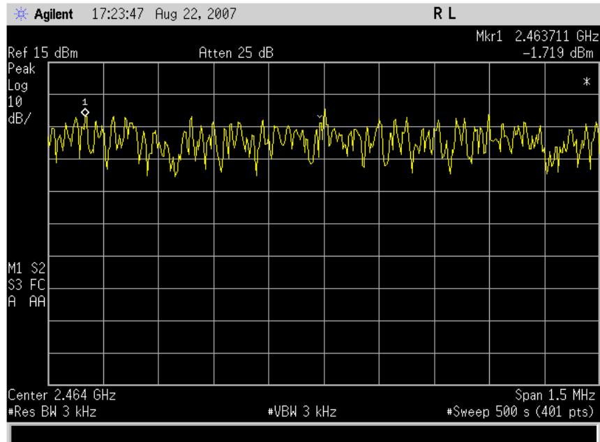
Peak Power Spectral Density, Channel 11
