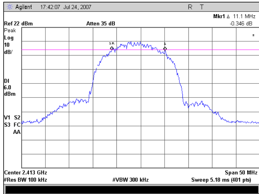
6 dB Occupied Bandwidth, Channel 1
