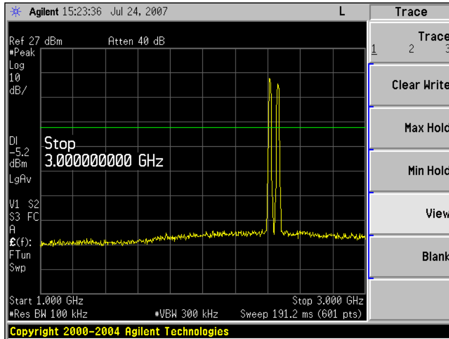
RF Conducted Spurious Emissions, 802.11b, 1-3 GHz
