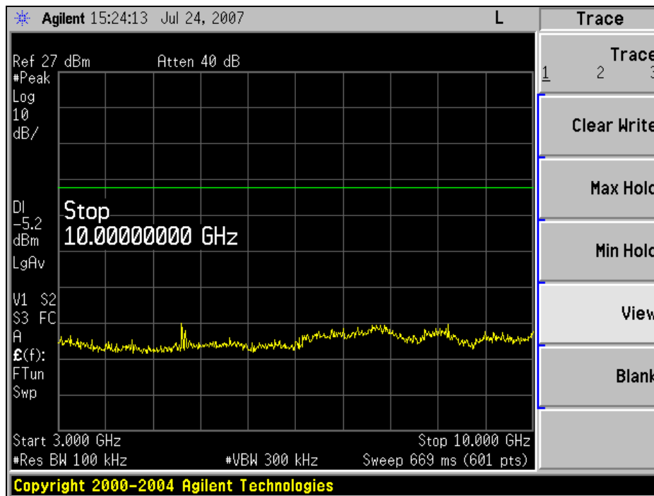
RF Conducted Spurious Emissions, 802.11b, 3-10 GHz
