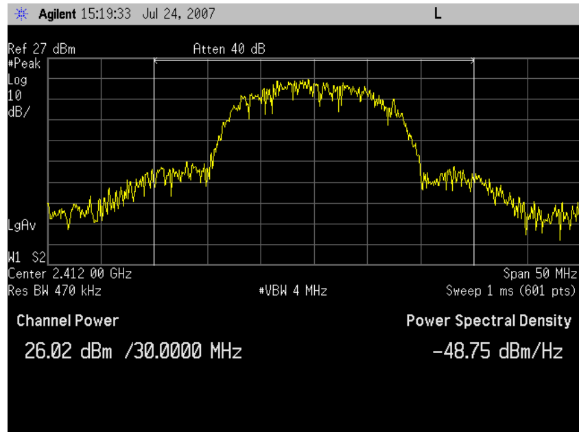
Peak Output Power, Channel 1
