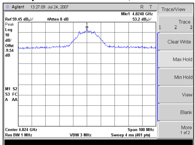
Spurious Radiated Emissions, 4.824 GHz, Peak
