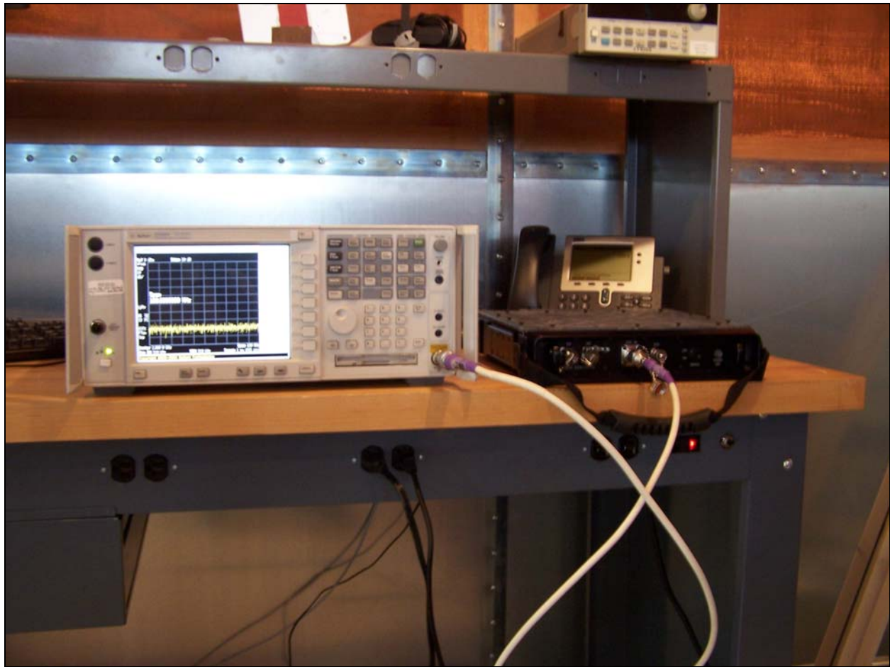
Photograph 4. 6 dB Bandwidth Test Setup
