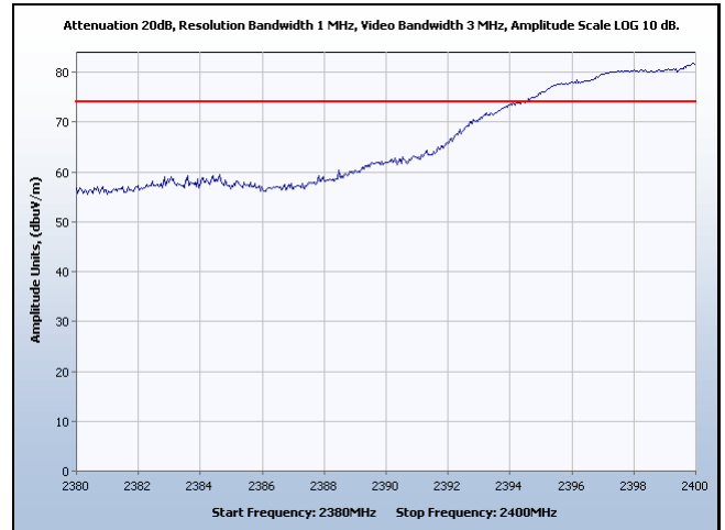
Restricted Band, Channel 1, Peak
