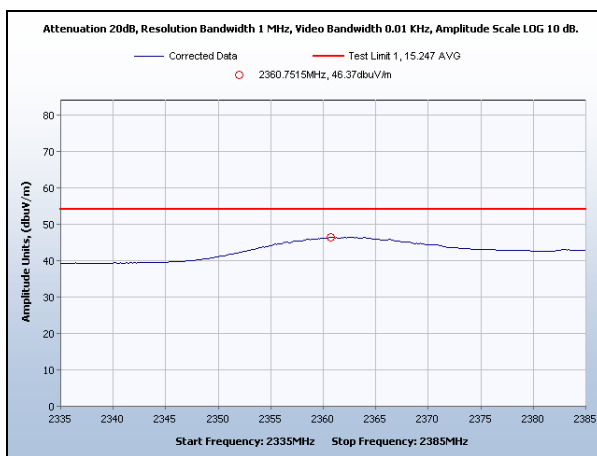
Restricted Band, 2360 MHz, Average
