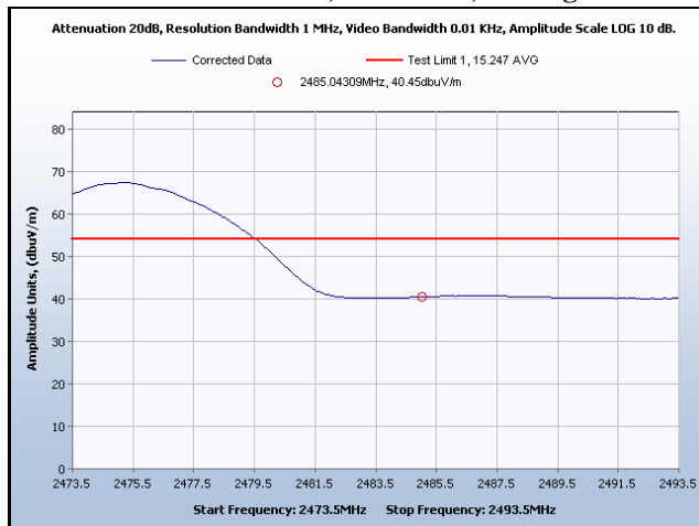
Restricted Band, Channel 11, Average
