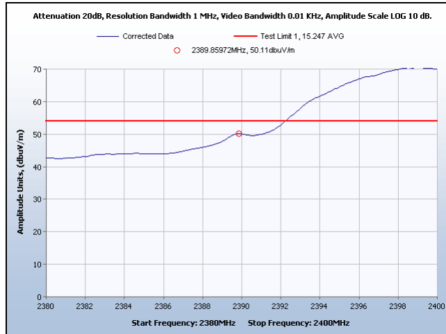
Restricted Band, Channel 1, Average
