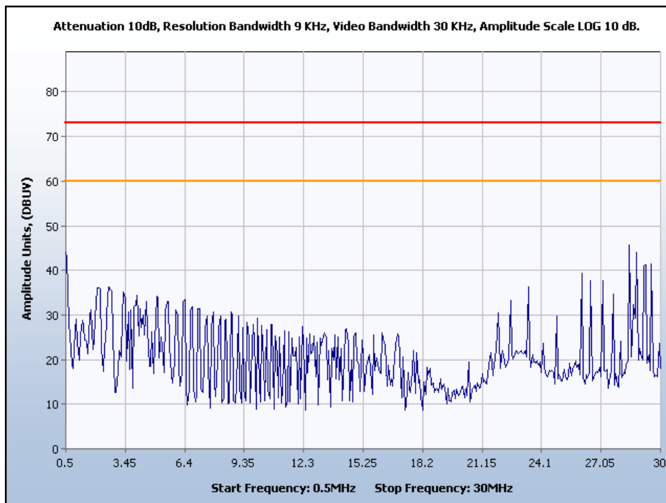
Phase Line Plot, 0.5 MHz to 30 MHz
