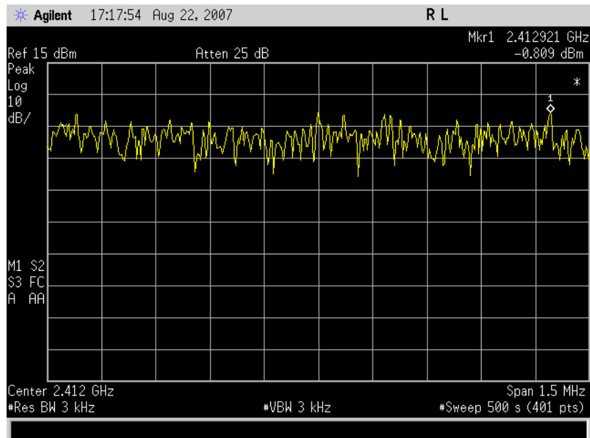
Peak Power Spectral Density, Channel 1
