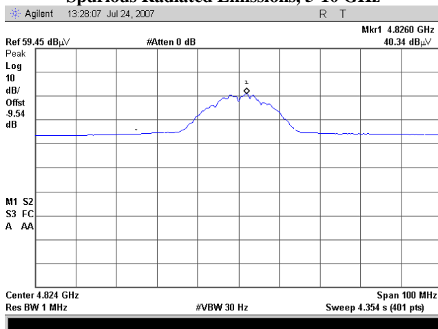
Spurious Radiated Emissions, 4.824 GHz Average
