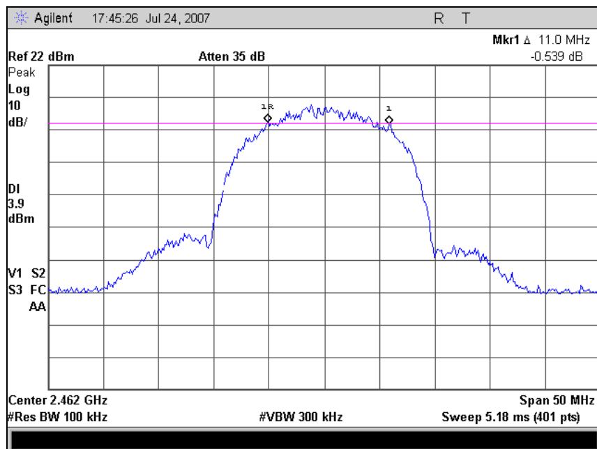
6 dB Occupied Bandwidth, Channel 11
