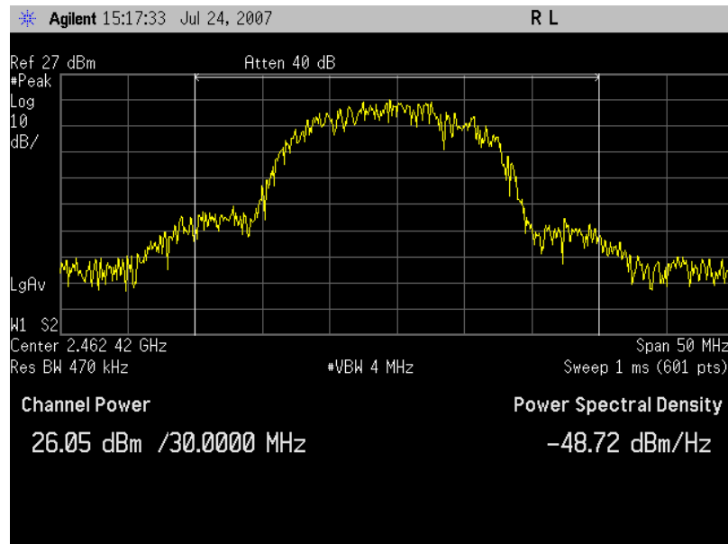
Peak Output Power, Channel 11
