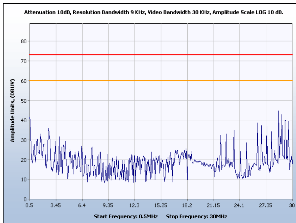
Neutral Line Plot, 0.5 MHz to 30 MHz
