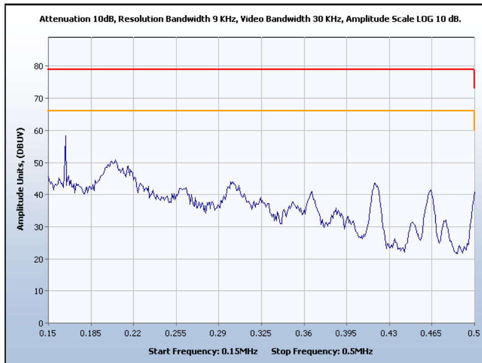
Neutral Line Plot, 0.15 MHz to 0.5 MHz
