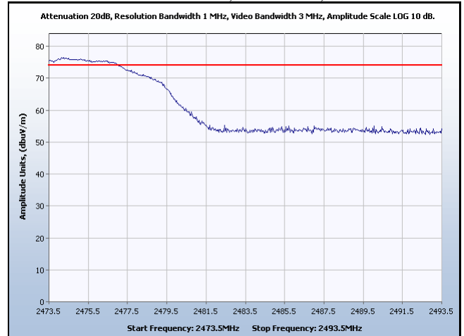
Restricted Band, Channel 11, Peak
