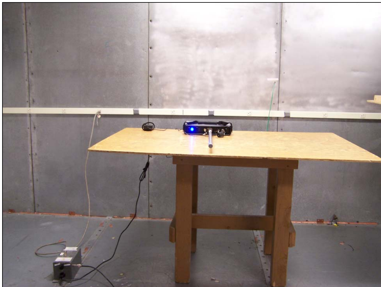
Photograph 2. Conducted Emission Test Setup
