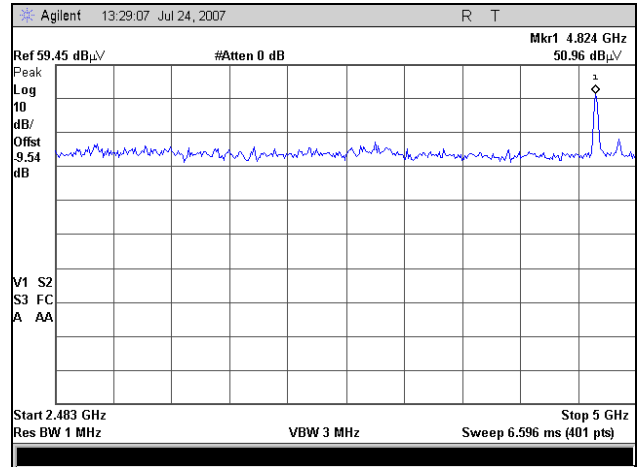
Spurious Radiated Emissions, 2.5 - 5 GHz
