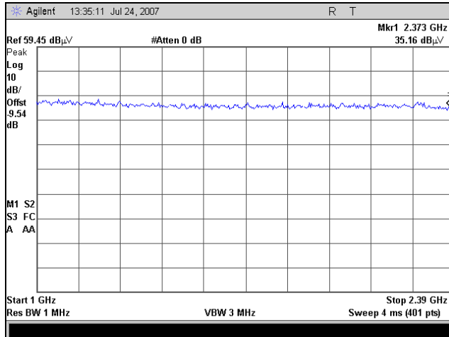
Spurious Radiated Emissions, 1 – 2.39 GHz
