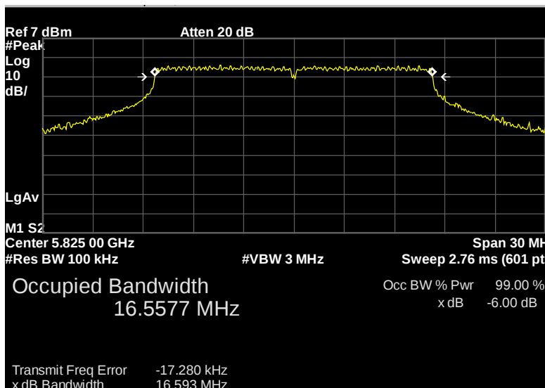
Figure 119: 6dB Occupied Bandwidth, 5825MHz, Chain 1
