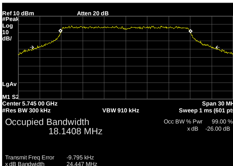
Figure 17: 26dB Bandwidth, n20, 5745MHz, Chain 1
