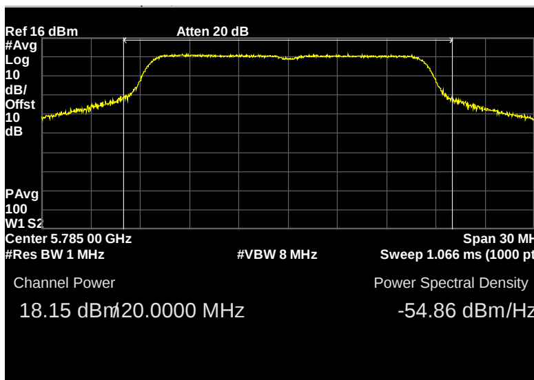
Figure 35: Output Power, 802.11a, 20MHz_5785MHz, Chain 1
