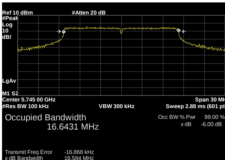
Figure 115: 6dB Occupied Bandwidth, 5745MHz, Chain 1
