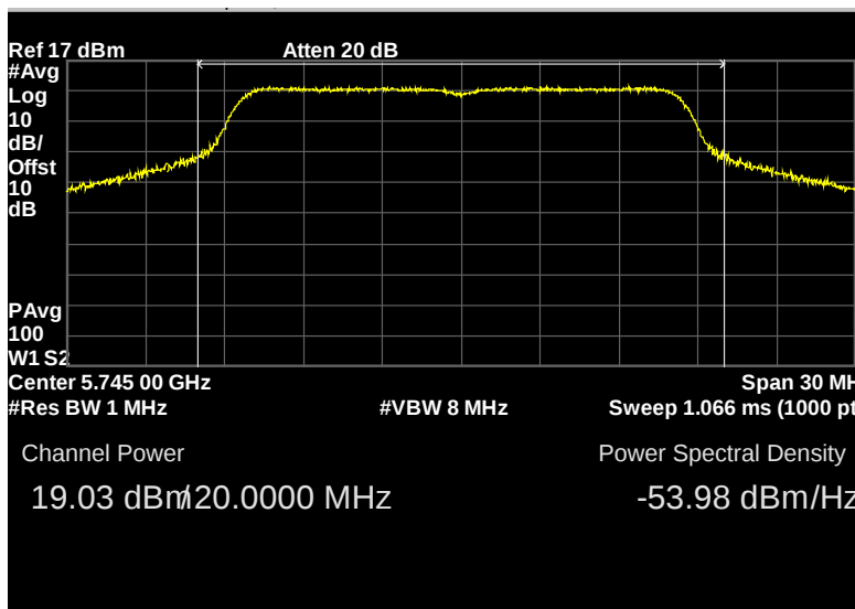
Figure 32: Output Power, 802.11a, 20MHz_5745MHz, Chain 0
