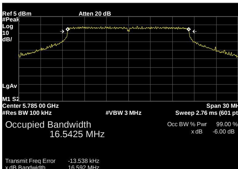
Figure 117: 6dB Occupied Bandwidth, 5785MHz, Chain 1
