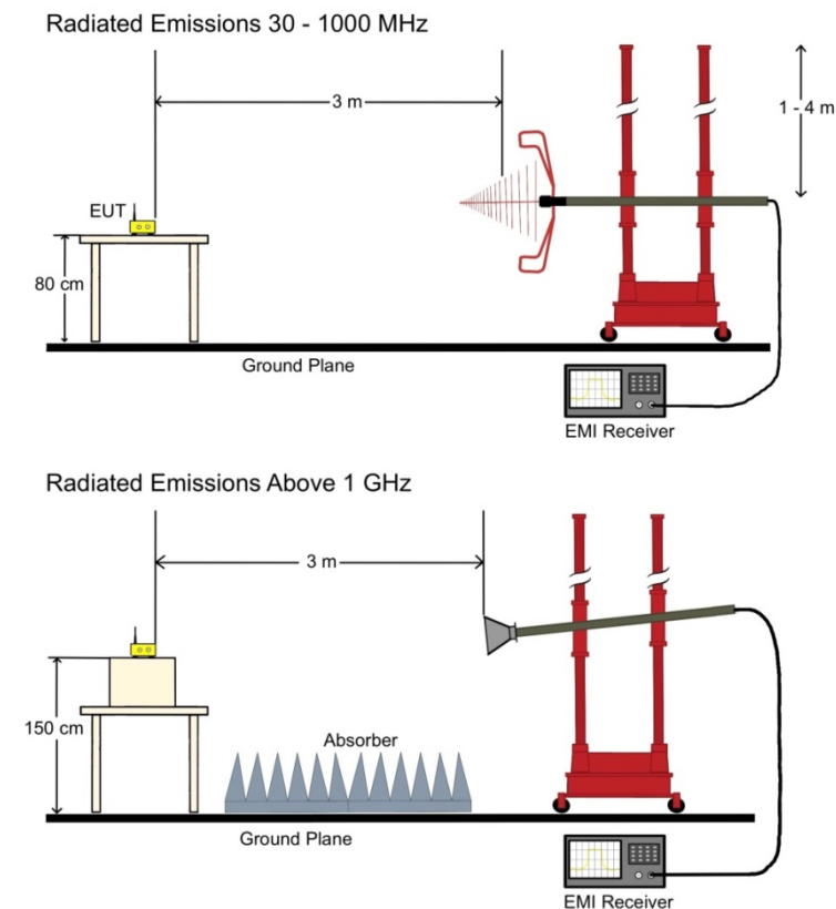
Figure 66: Radiated Emissions Test Setup
