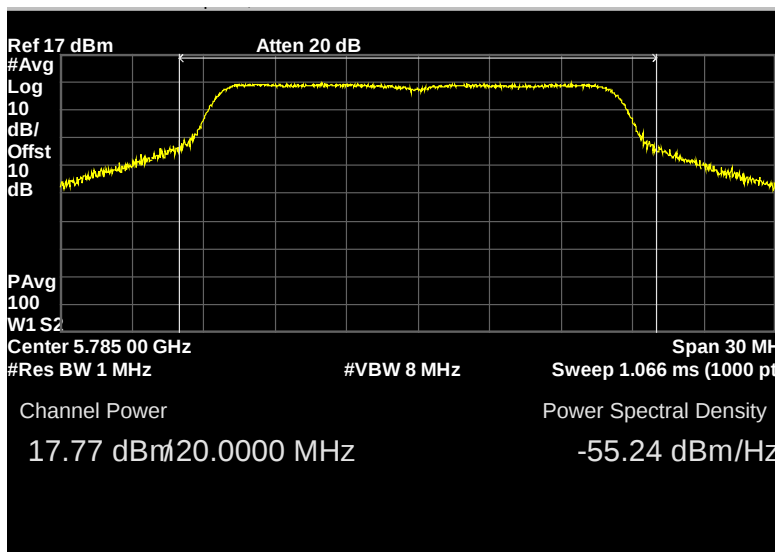
Figure 34: Output Power, 802.11a, 20MHz_5785MHz, Chain 0
