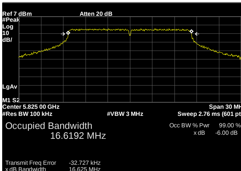
Figure 118: 6dB Occupied Bandwidth, 5825MHz, Chain 0
