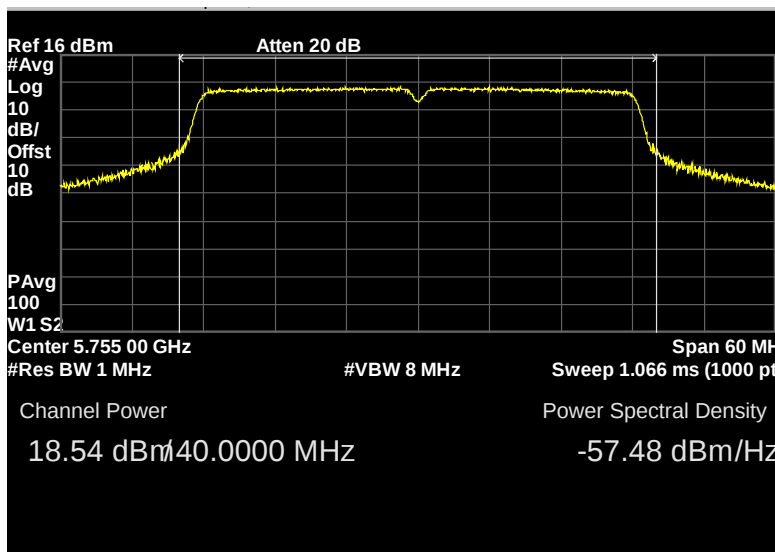
Figure 44: Output Power, 802.11n, 40MHz_5755MHz, Chain 0
