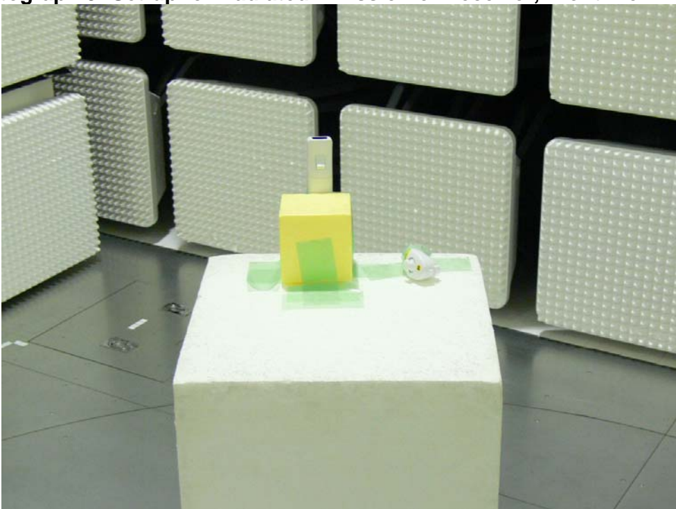
Photograph 9: Set-up for Radiated Emission of Receiver, Front View
