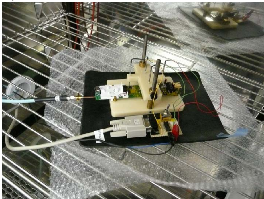
Photograph 3: Set-up for AC Mains Conducted Emission of Transmitter, Front View
