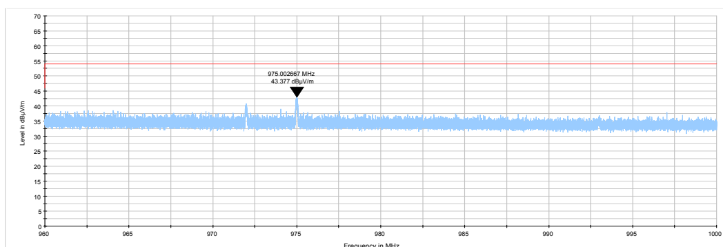
Plot 7.3.13 Radiated emission measurements from 960-1000 MHz at the high carrier frequency
