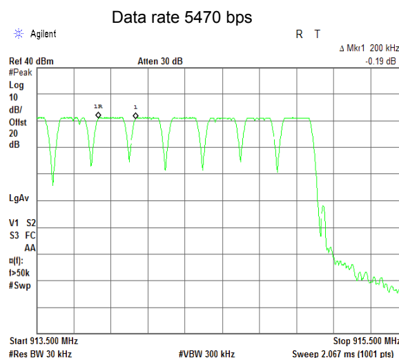
Plot 7.2.1 Carrier frequency separation
