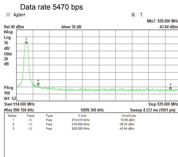
Plot 7.8.2 The highest band edge emission at high carrier frequency with hopping function disabled
