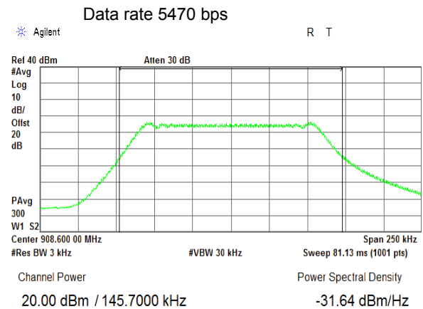
Plot 7.5.2 Peak output power at mid frequency
