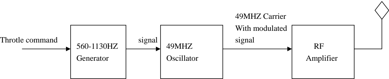
49MHZ Product Block Diagram
