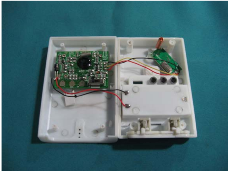
Photo 2- Front view of RF Module board
