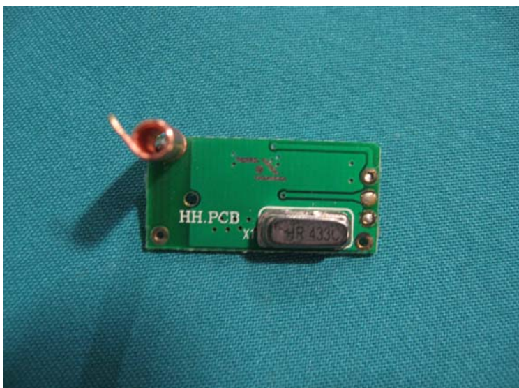
Photo 3 – Back view of RF Module board
