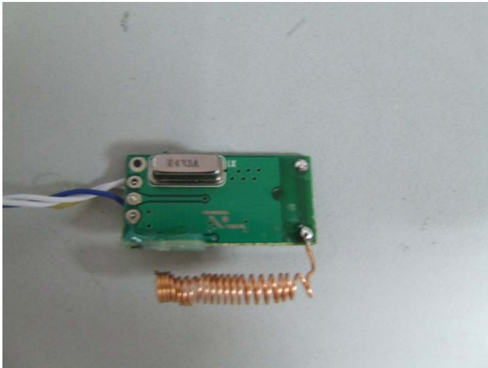
Photo 4-Front view of RF Main Board
