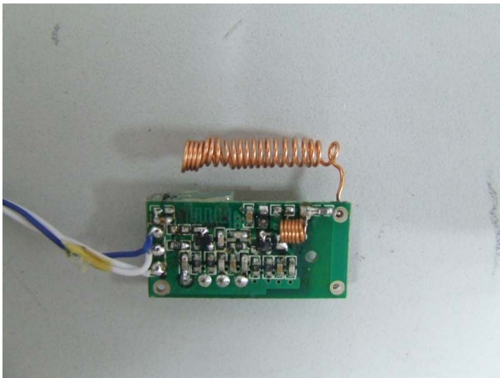
Photo 2-Front view of RF Module Board
