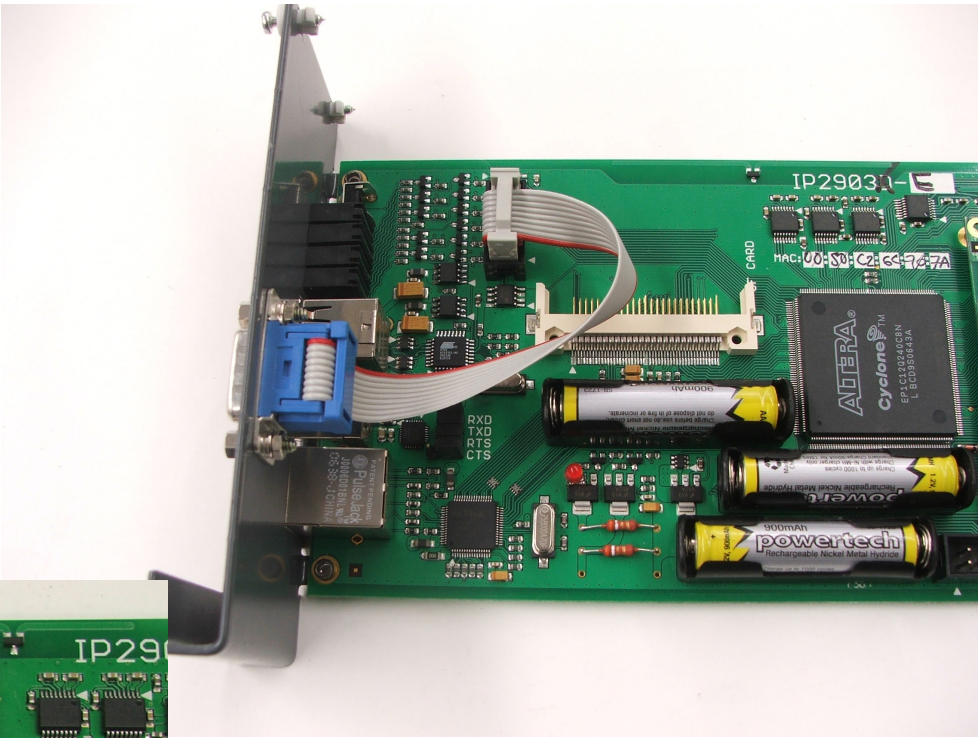
Close up of front adjacent to cover plate with Flash memory fitted removed.
