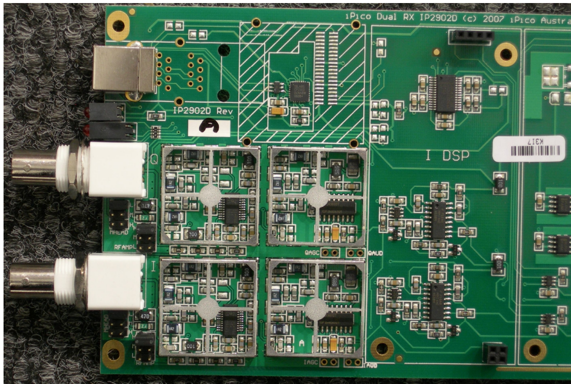
Figure 3 IP2902 Top view with component shields removed
