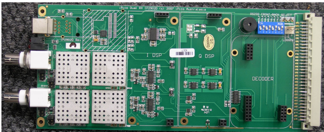
Figure 2 IP2902 Receiver top view
