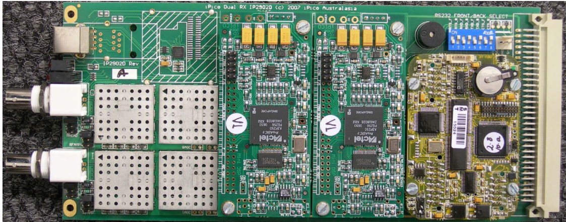
Figure 1 Receiver module fitted with DSP and Decoder modules
