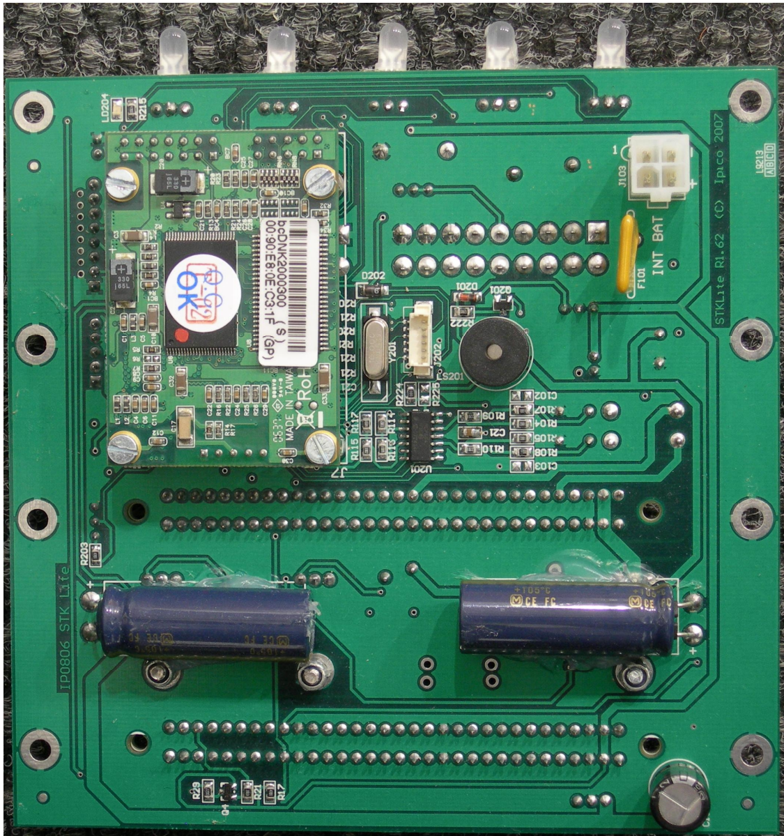
Figure 3 IP0806 with MOXA IP0679 fitted
