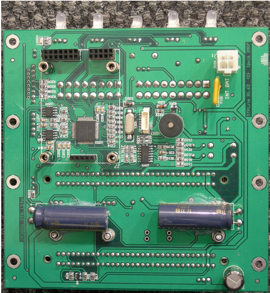
Figure 2 IP0806 Bottom view
