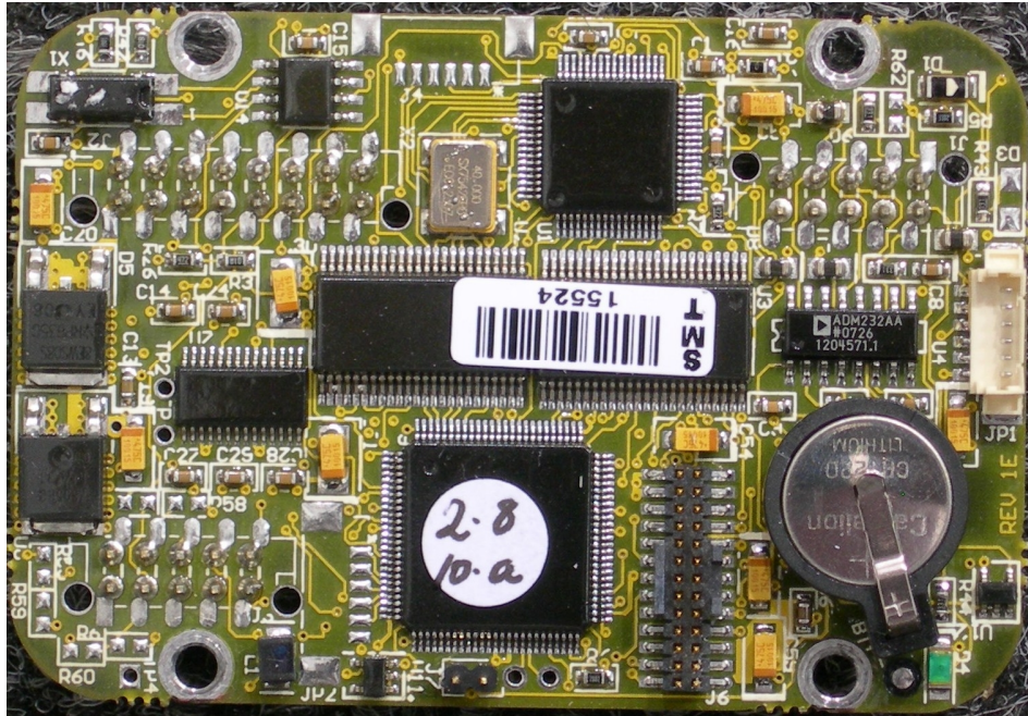
Figure 1 IP2176 Top view
