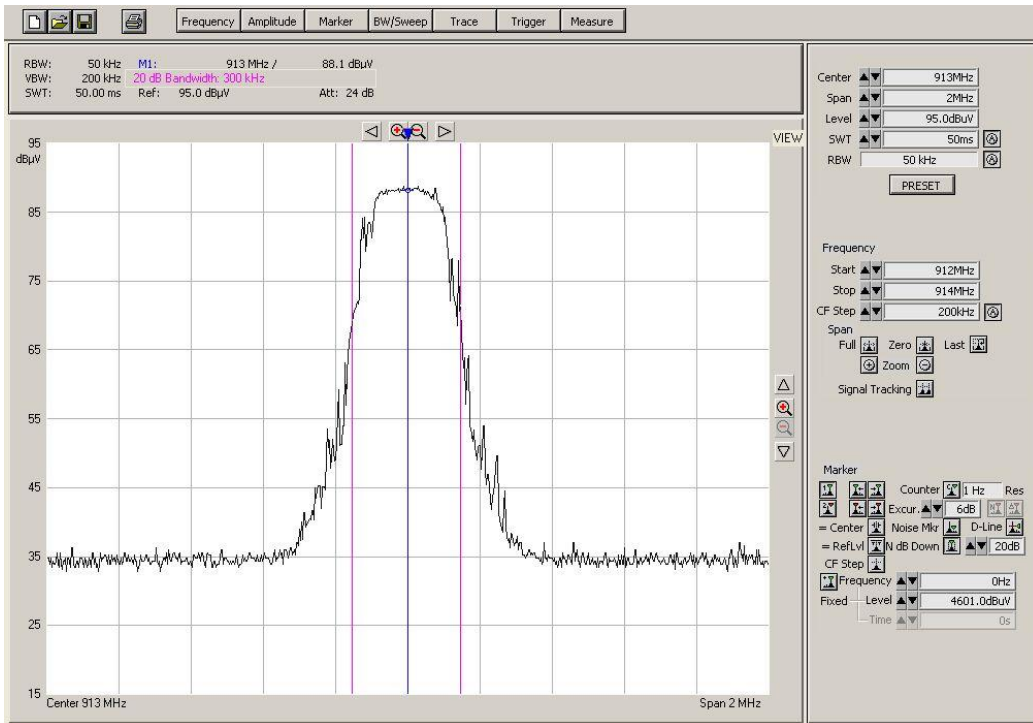
Channel 2 – 20 dB point, Bandwidth 300 kHz
