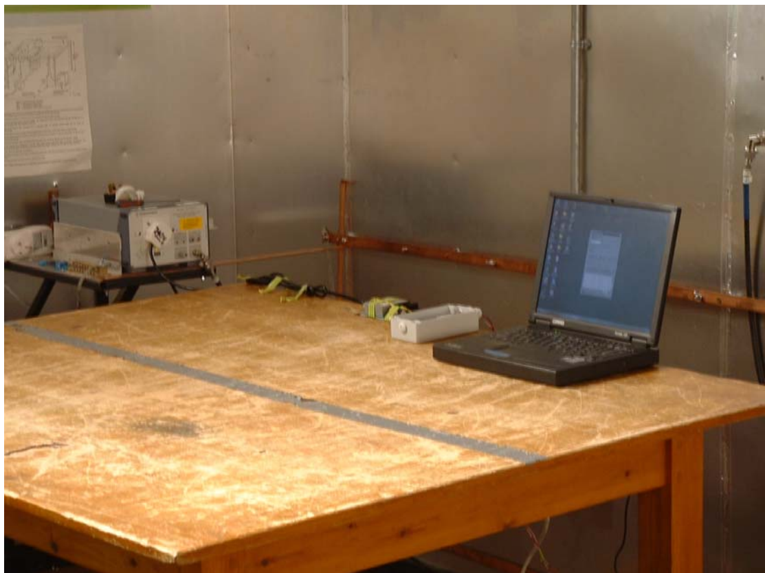
AC Powerline Conducted Emissions Test Setup
