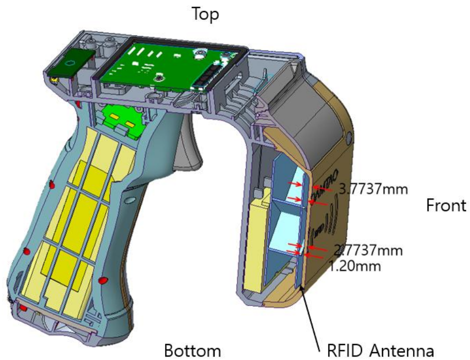
Figure E-1 Antenna Location
