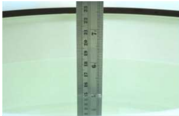
Figure D-1 Liquid Height for Body Position (SAM Phantom)
