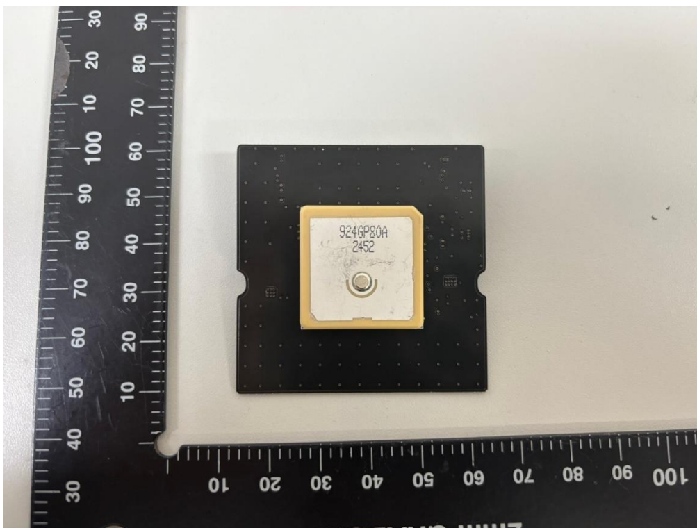
RFID Ceramic Patch Antenna
