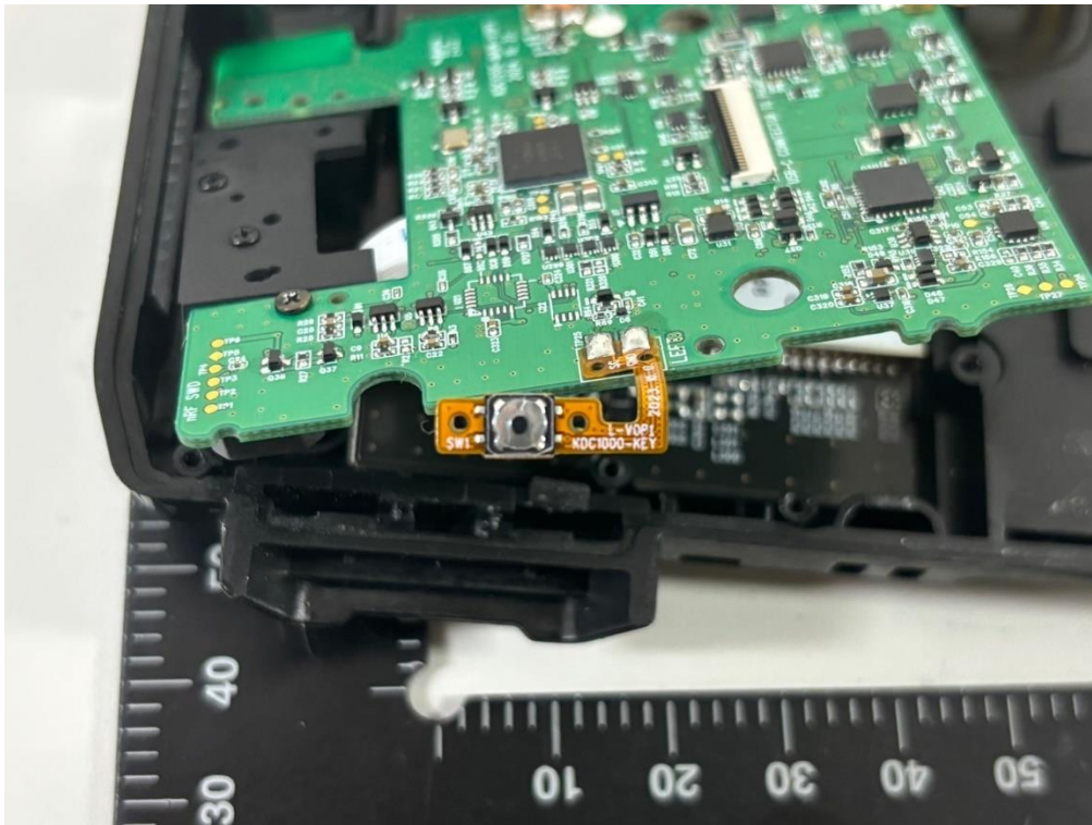
Button Pcb Board
