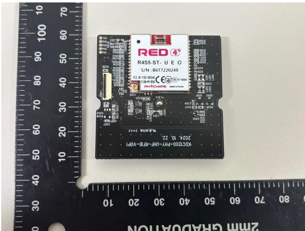
RFID Module Shield can – Front
