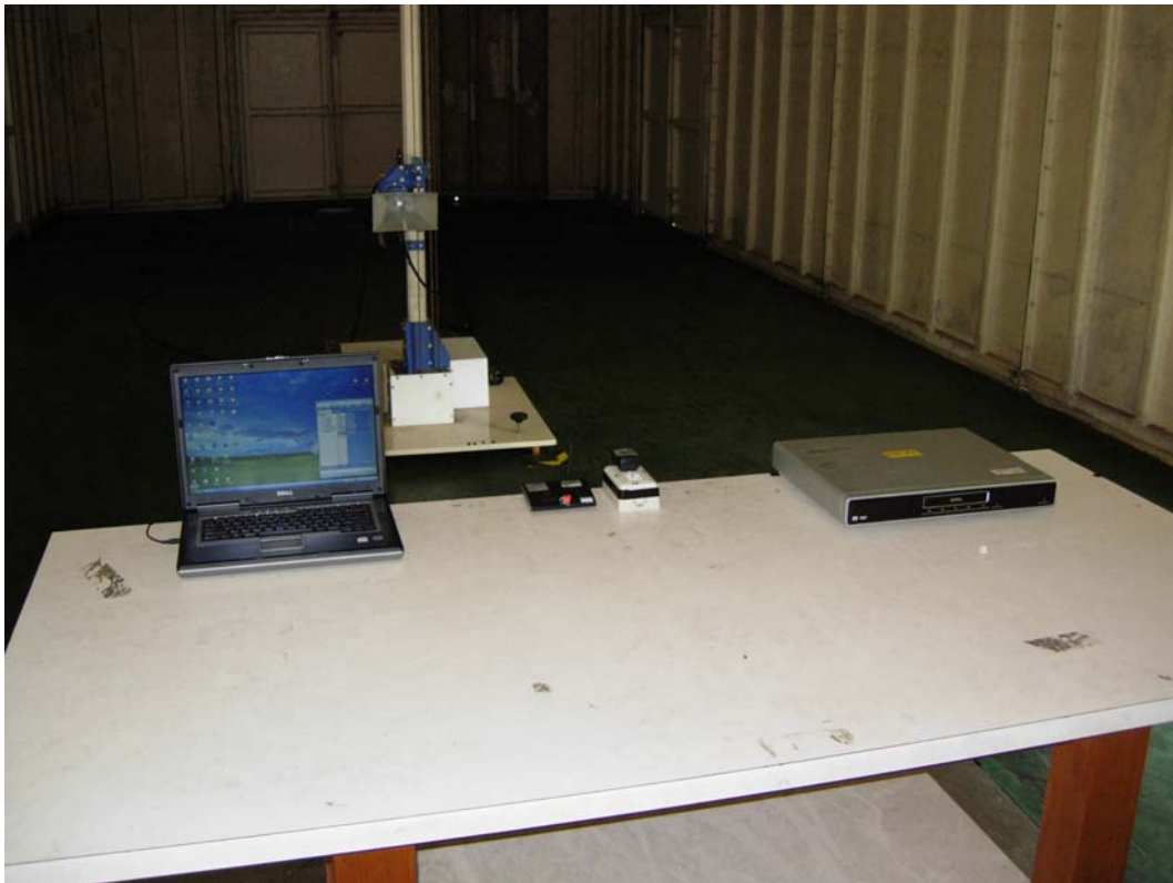
Back View of Radiated Test (Horn) – Mode 1
