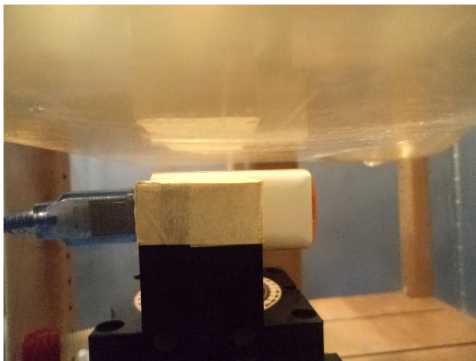
Vertical-Front Setup Photo (0.5cm)
