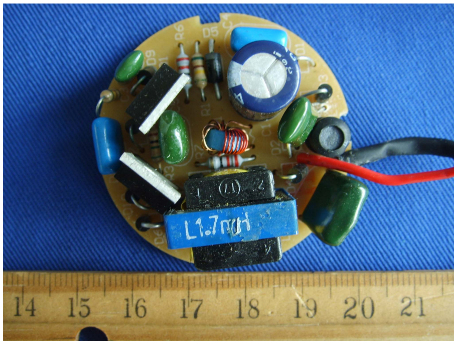
EUT –Components View (GY PL26W)
