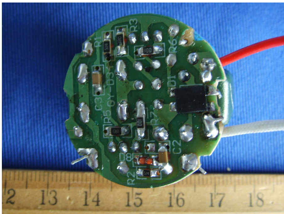
EUT–Solder View (GY PL18W)
