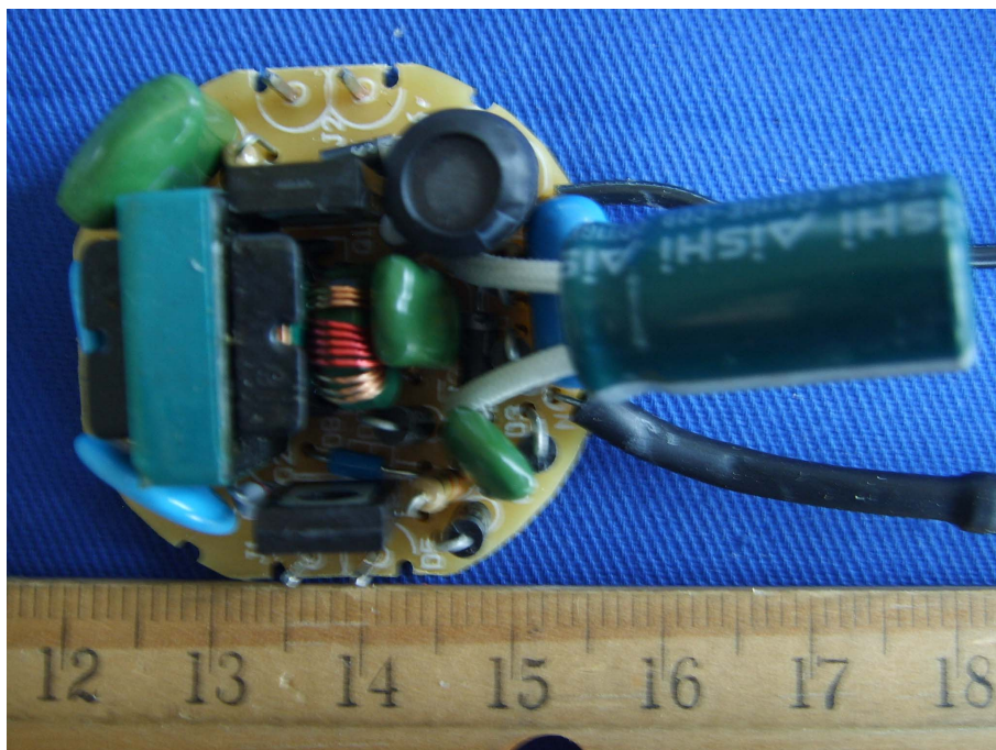
EUT –Components View (GY T3S18WE26)
