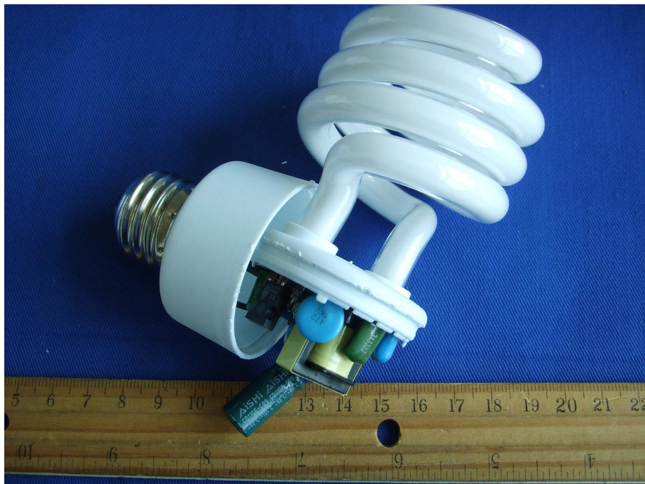
EUT – Uncovered View (GY T3S23WE26)
