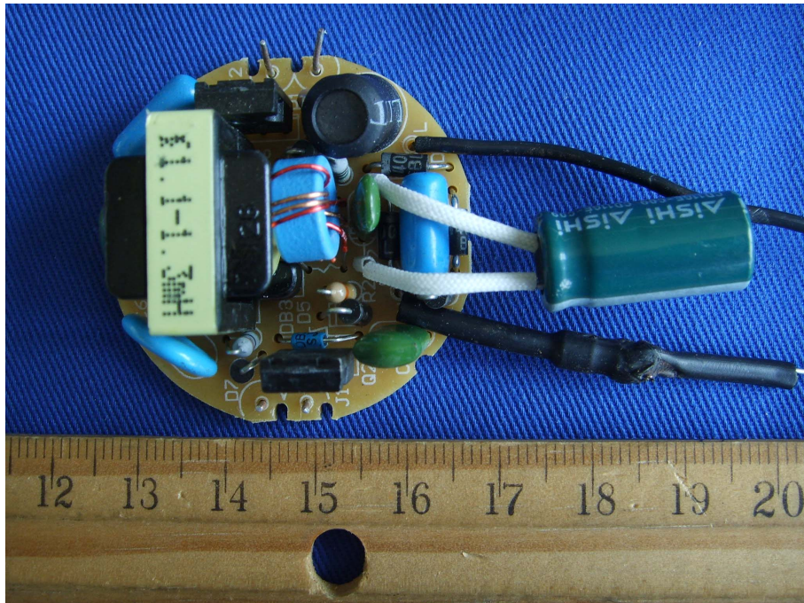
EUT –Components View (GY T3S23WE26)
