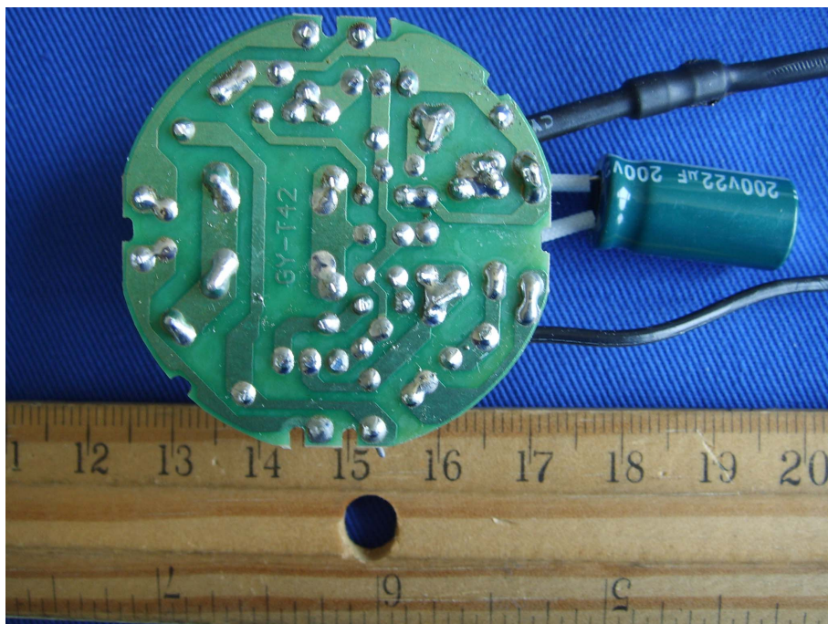
EUT–Solder View (GY T3S23WE26)
