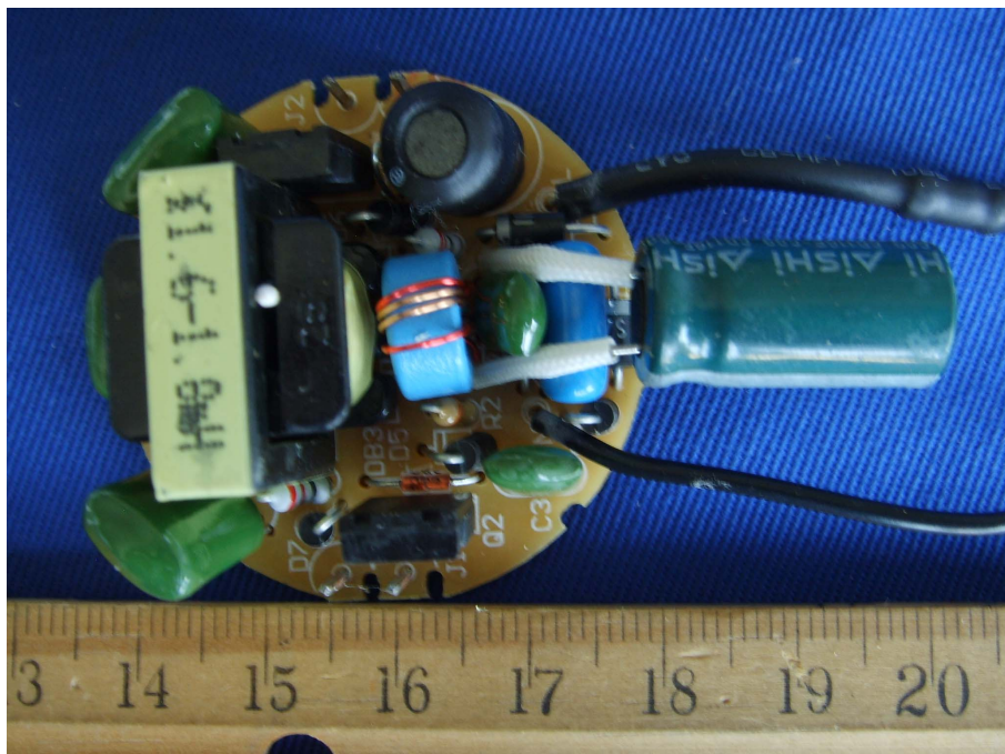
EUT –Components View (GY T3S25WE26)
