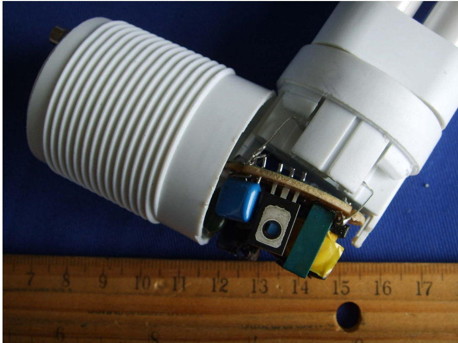
EUT – Uncovered View (GY PL13W)
