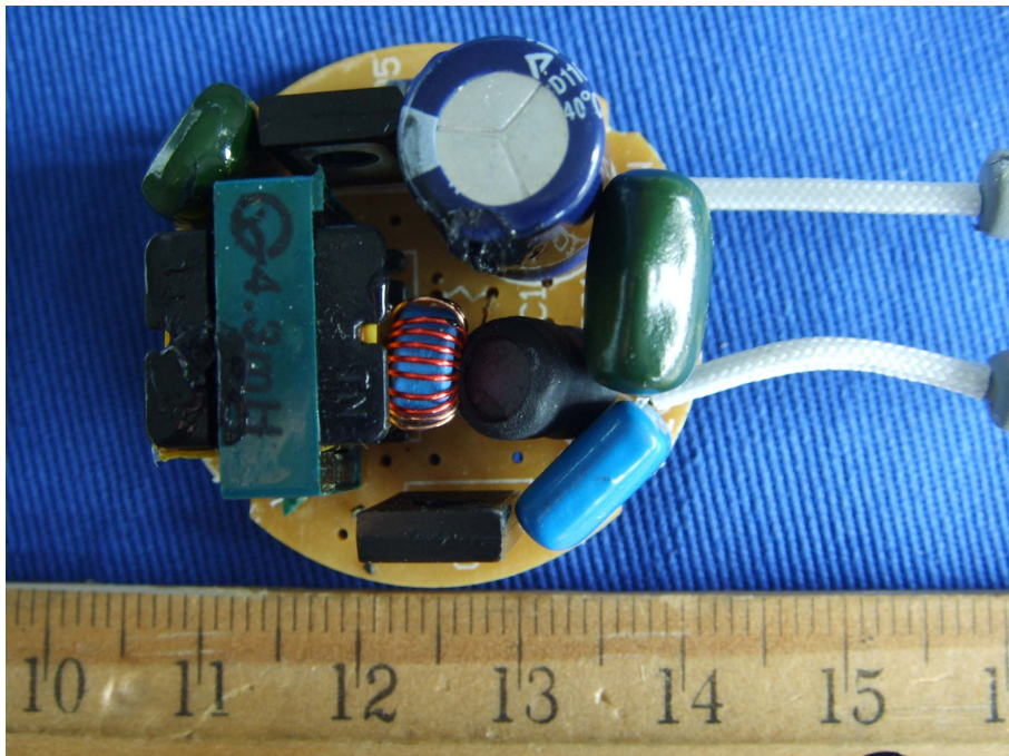
EUT –Components View (GY PL13W)
