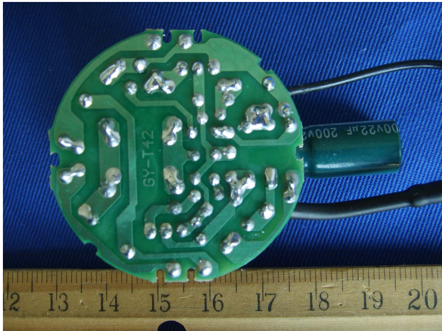
EUT–Solder View (GY T3S25WE26)
