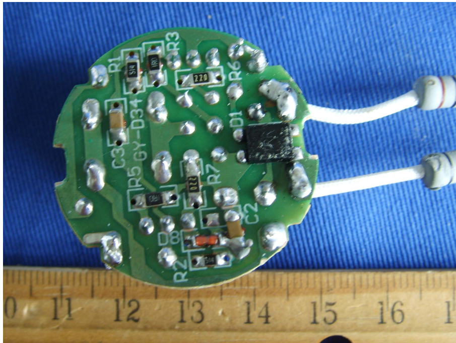
EUT-Solder View (GY PL13W )
