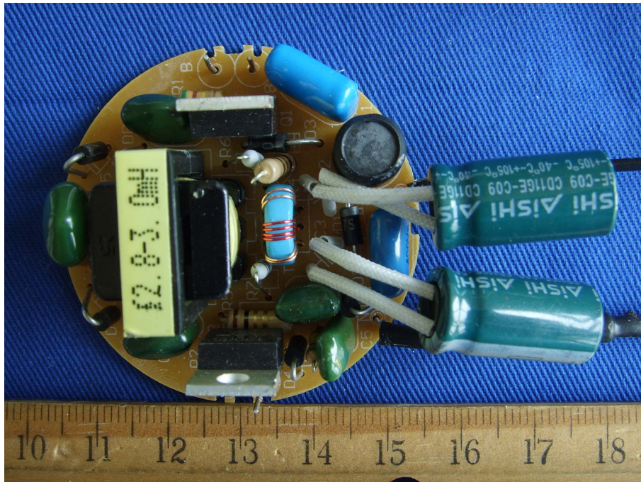
EUT –Components View (GY T3S30WE26)
