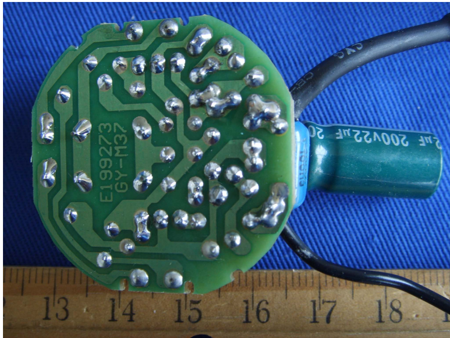
EUT–Solder View (GY T3S18WE26)
