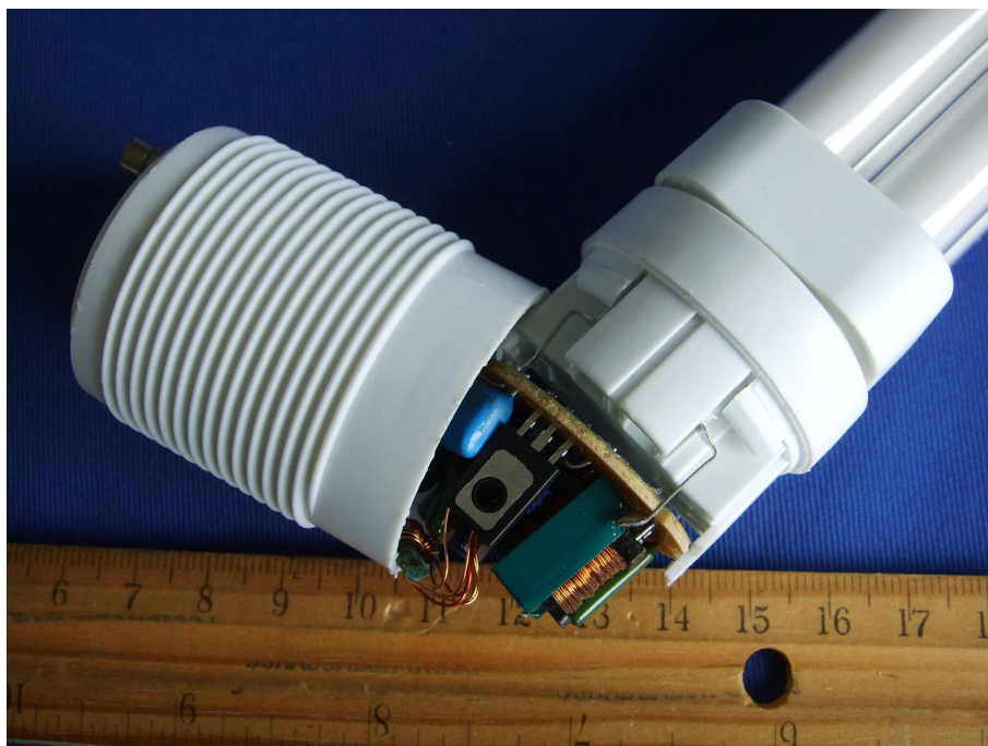
EUT – Uncovered View (GY PL18W )
