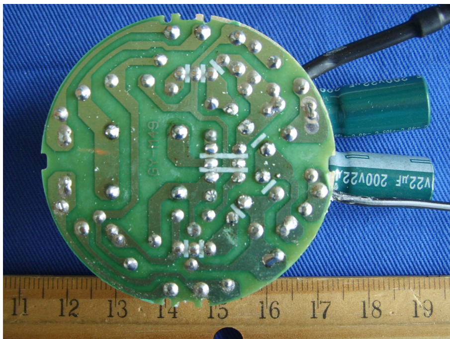
EUT –Solder View (GY T3S30WE26)
