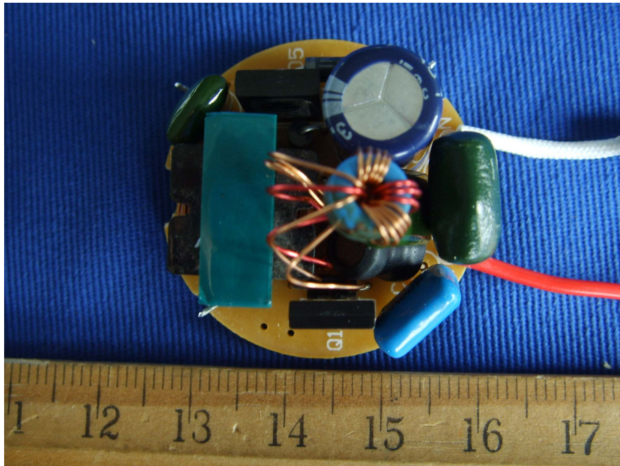
EUT –Components View (GY PL18W)
