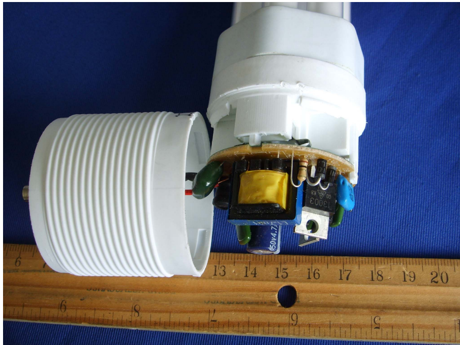
EUT – Uncovered View (GY PL26W)
