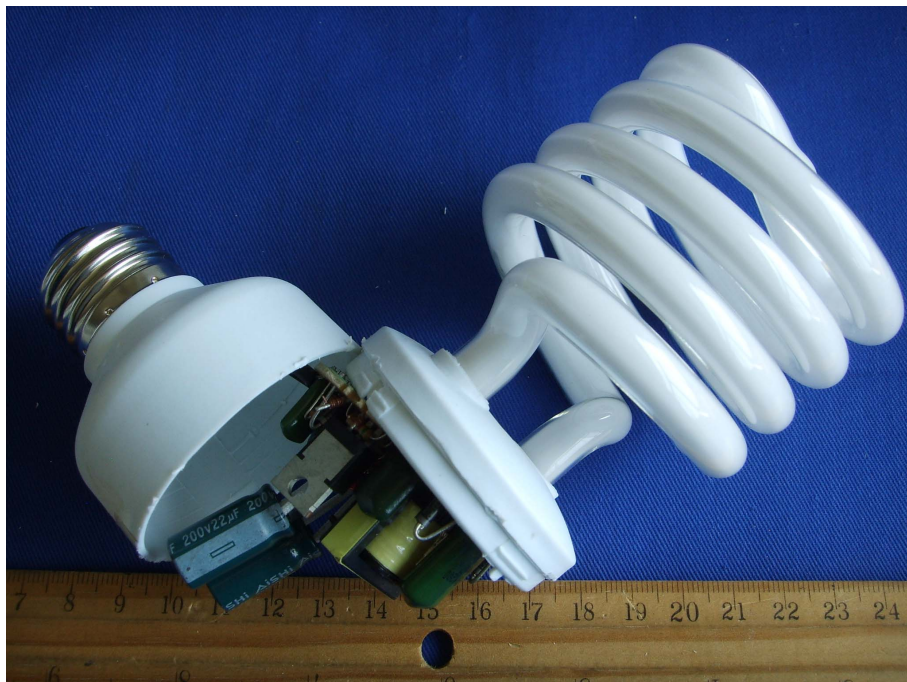
EUT – Uncovered View (GY T3S30WE26)
