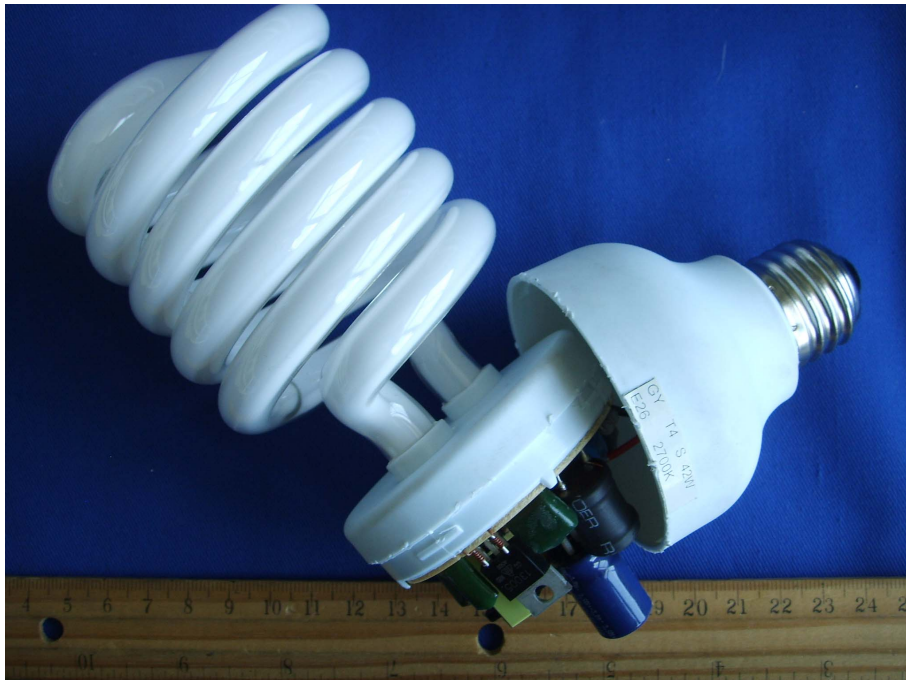
EUT – Uncovered View (GY T4S42WE26)
