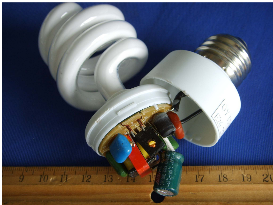
EUT – Uncovered View (GY T3S13WE26)
