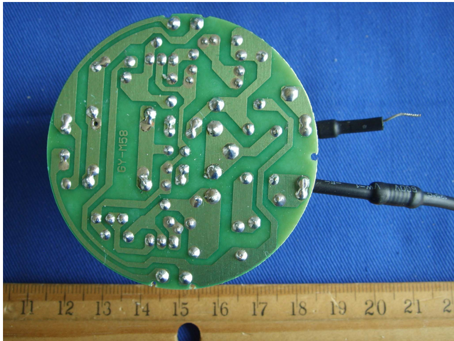
EUT–Solder View (GY T4S42WGU24)
