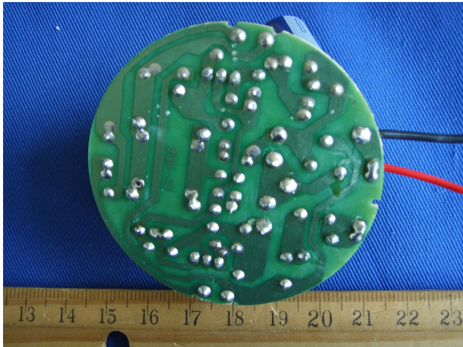
EUT–Solder View (GY T4S42WE26)
