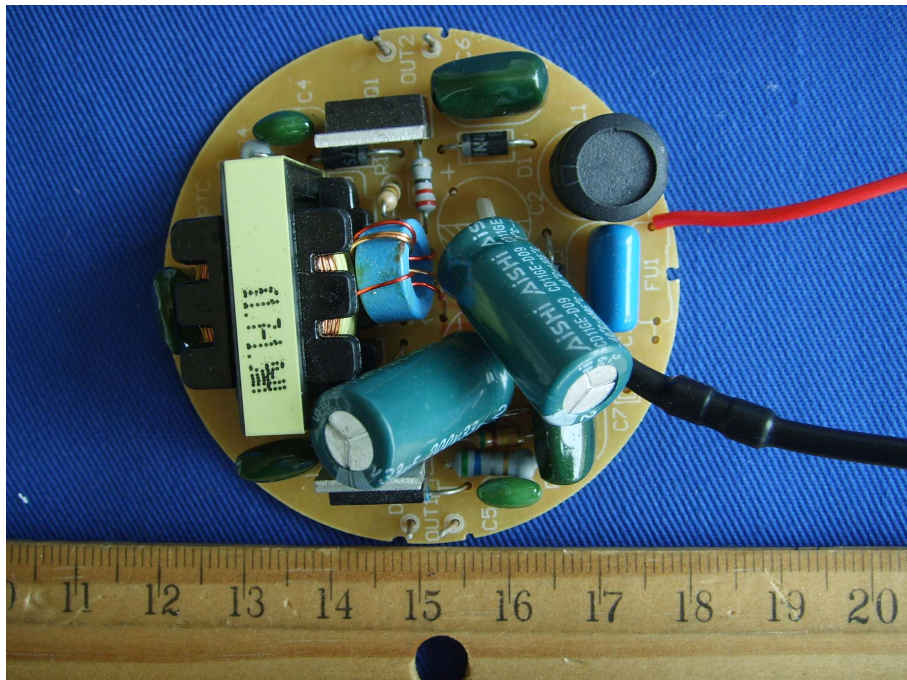
EUT –Components View (GY T4S32WGU24)
