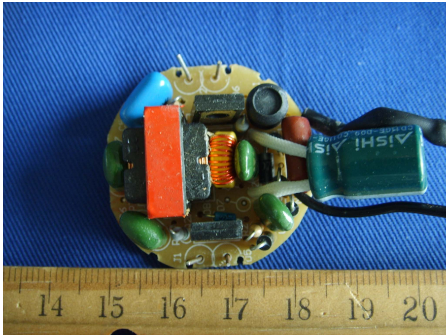
EUT –Components View (GY T3S13WE26)
