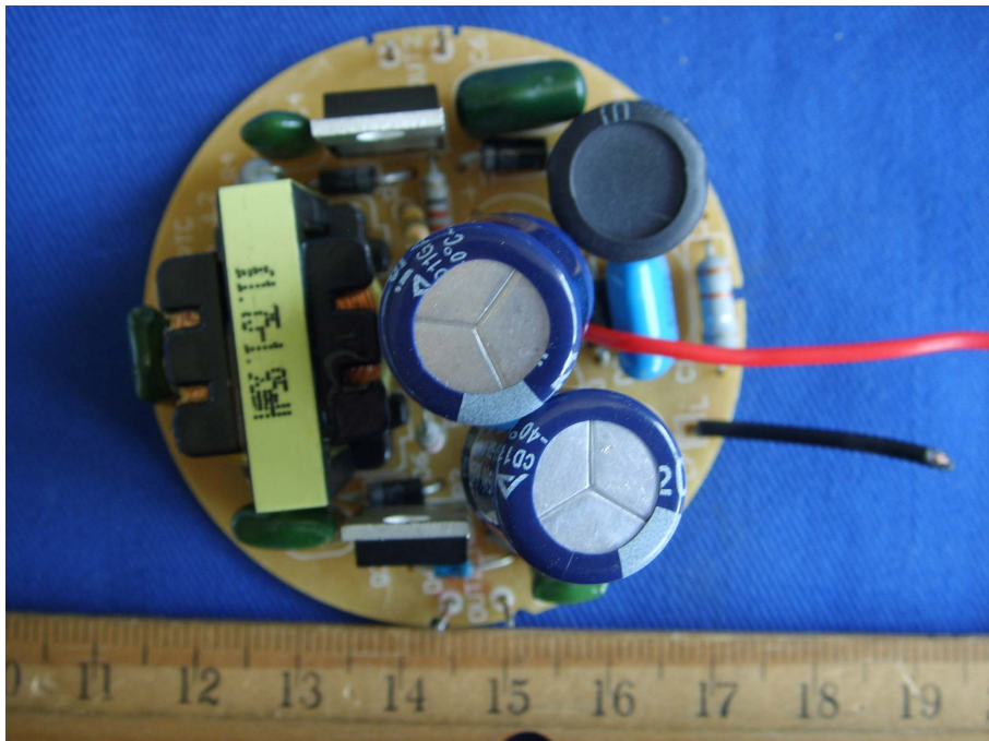
EUT –Components View (GY T4S42WE26)
