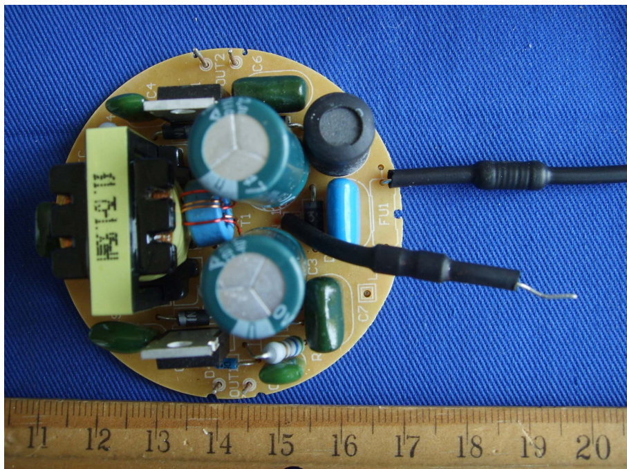
EUT –Components View (GY T4S42WGU24)
