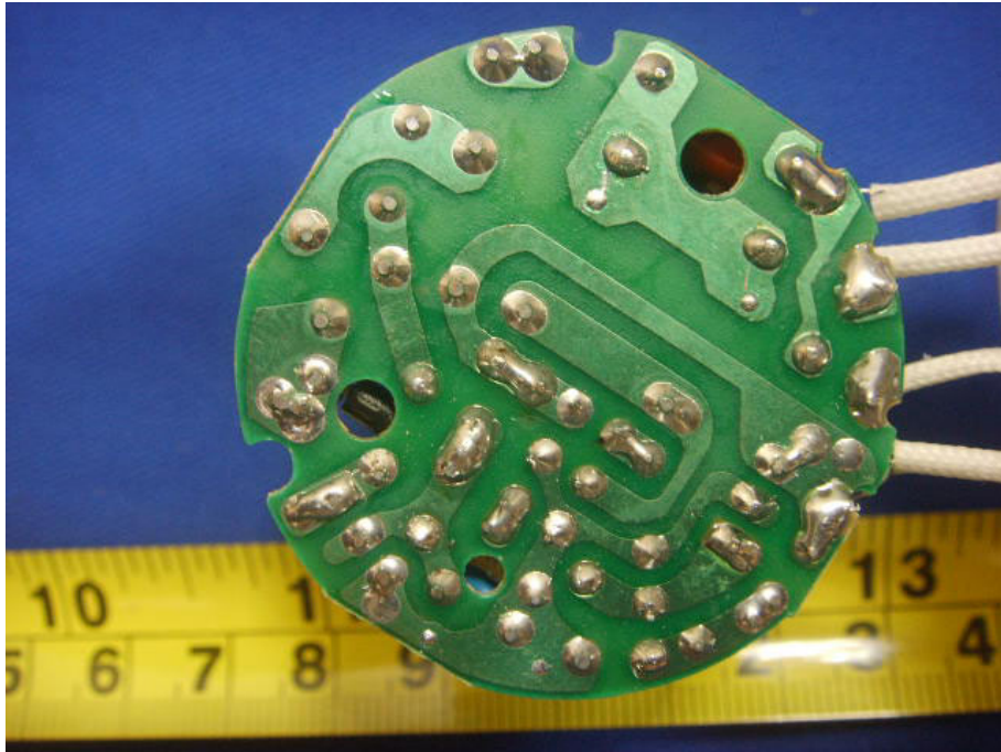
EUT–Solder View (SCE-23W)
