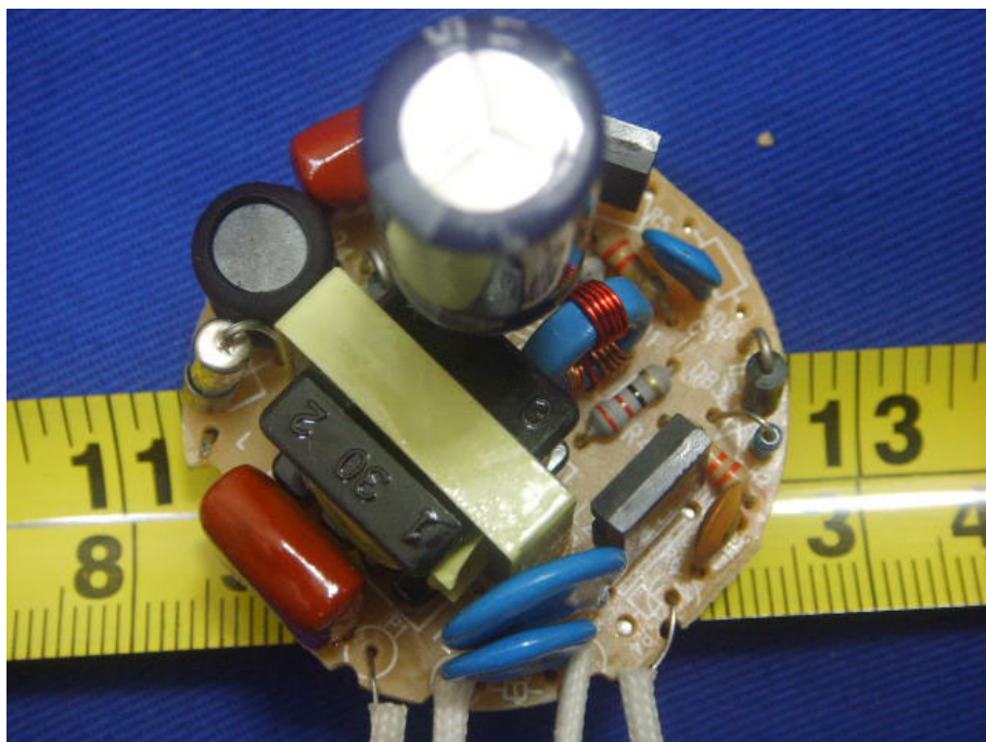
EUT –Components View (SCE-23W)
