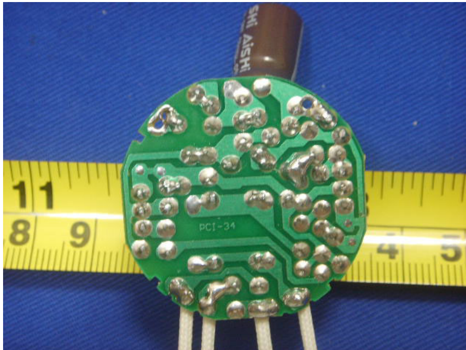
EUT–Solder View (SEM-13W)
