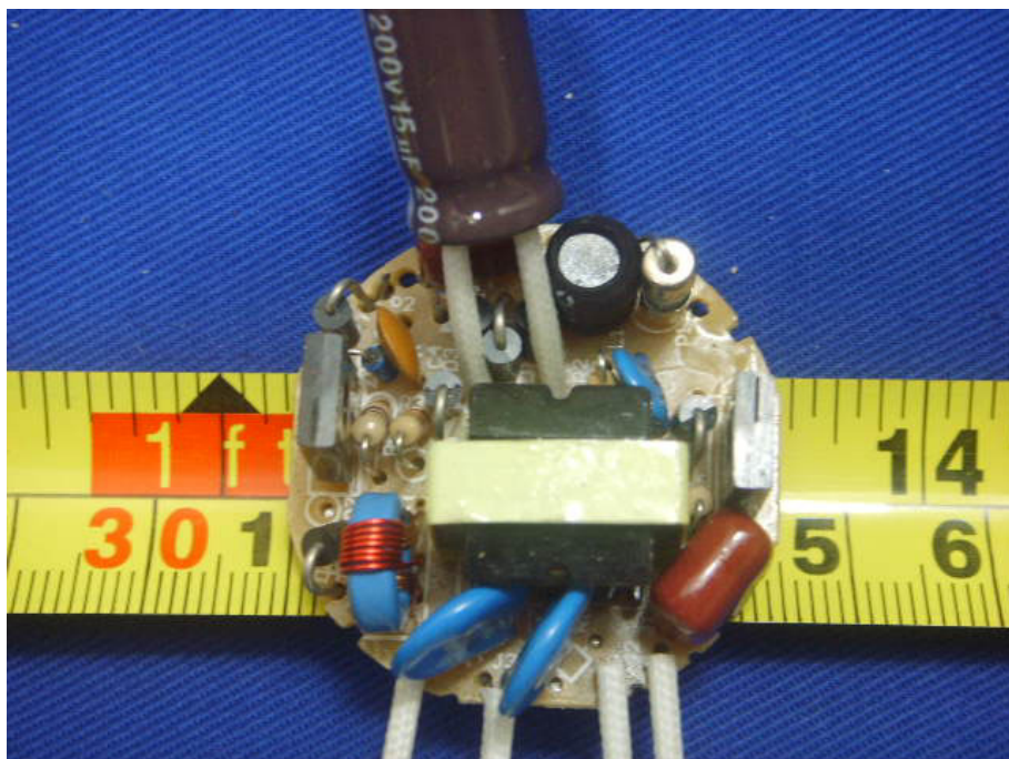
EUT –Components View (SEM-13W)
