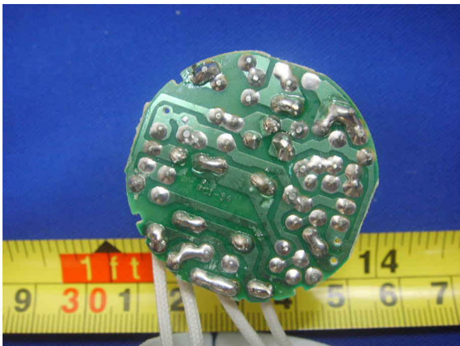
EUT–Solder View (SEM-9W)
