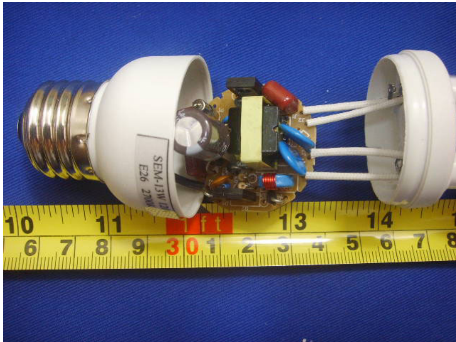
EUT – Uncovered View (SEM-13W)
