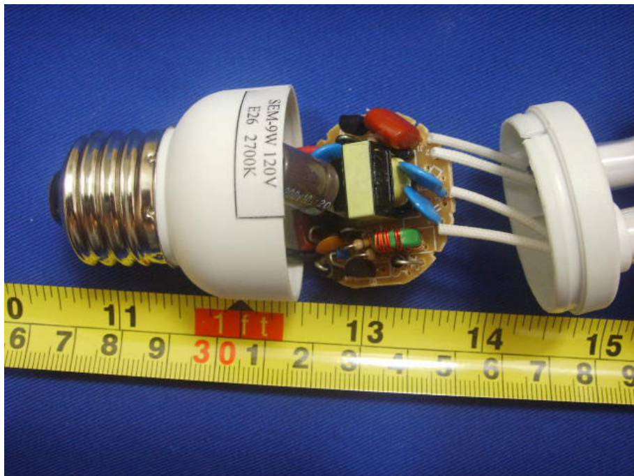
EUT – Uncovered View (SEM-9W)
