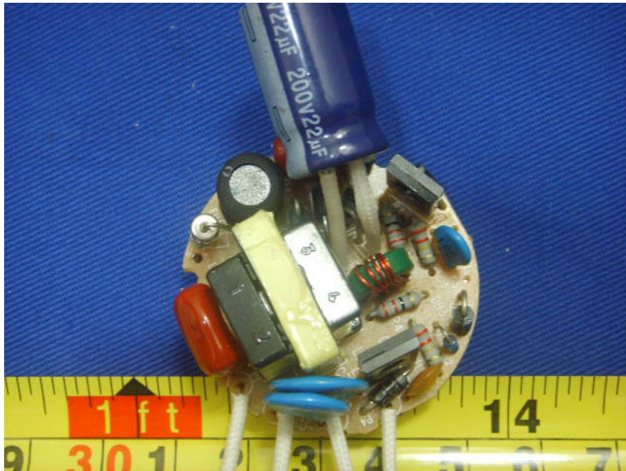
EUT –Components View (SCE-20W)
