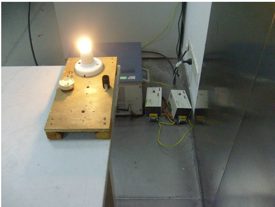
GYT2S03-E26: Conducted Emissions - Side View
