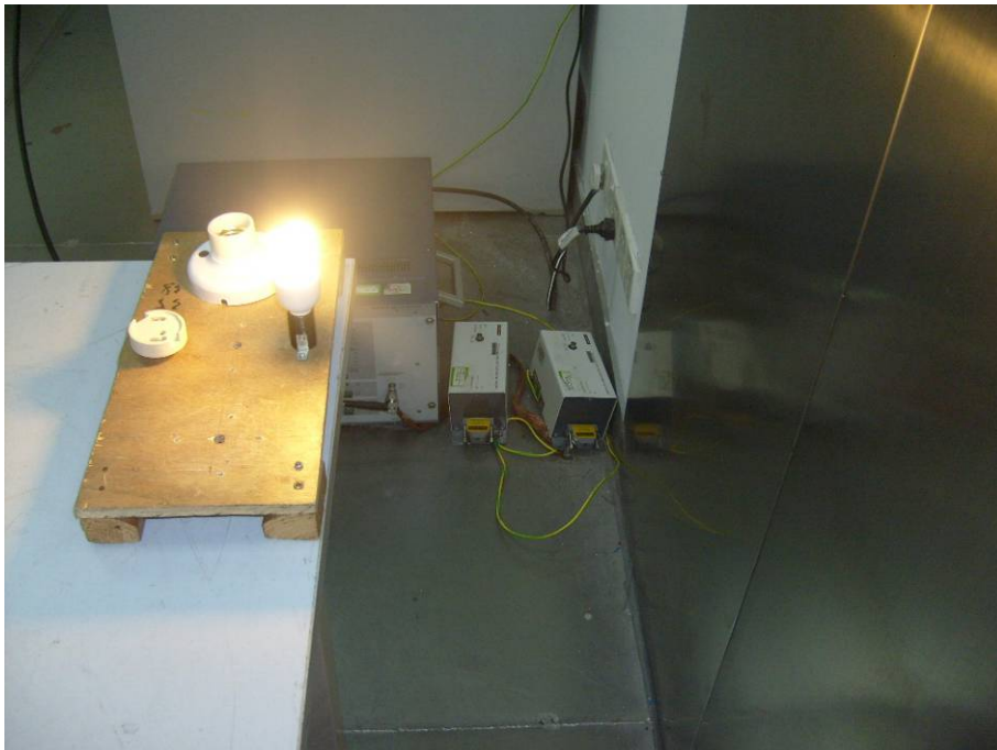
GYT2S07-E12: Conducted Emissions - Side View
