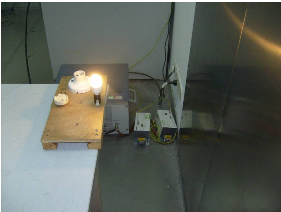
GYT2S03-E12: Conducted Emissions - Side View
