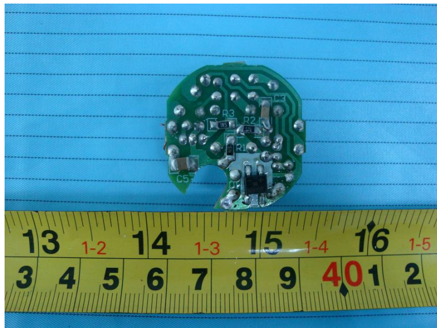
GYC05-E26: EUT – Main Board Bottom View
