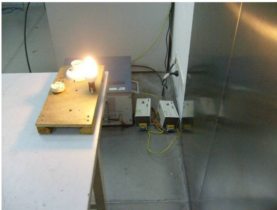
GYC07-E12: Conducted Emissions - Side View
