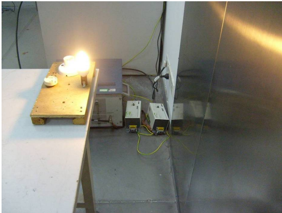
GYC05-E12: Conducted Emissions - Side View
