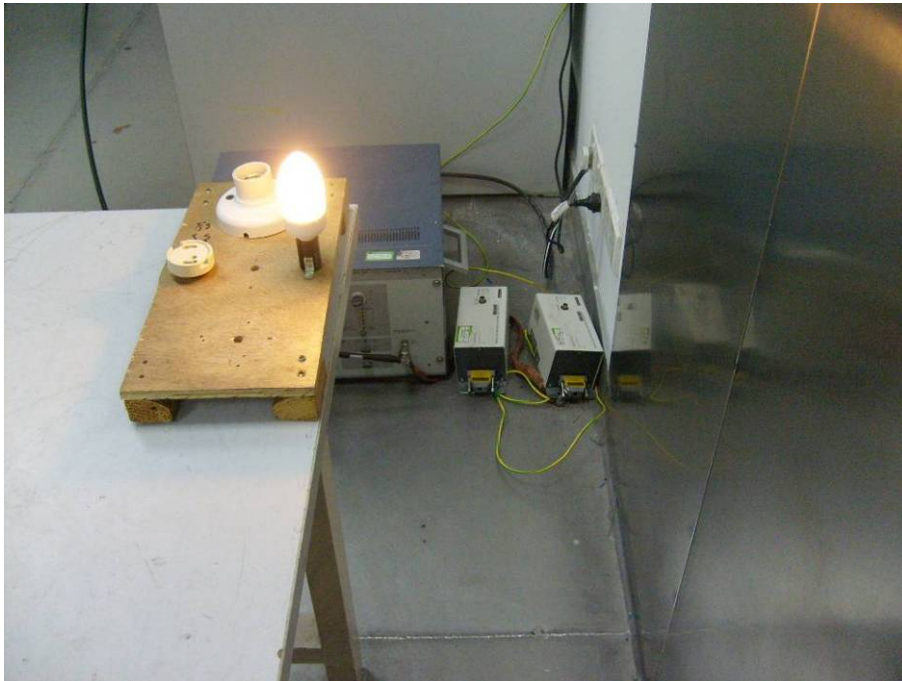
GYC03-E12: Conducted Emissions - Side View
