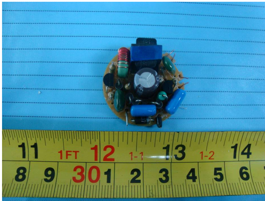
GYC03-E12: EUT – Main Board Top Components View
