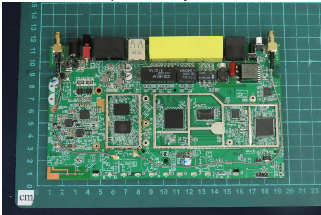
(42) EUT Photo - Brand Name: DrayTek, Model No.: Vigor2767Vax
