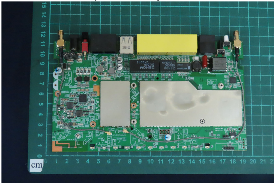
(40) EUT Photo - Brand Name: DrayTek, Model No.: Vigor2767Vax
