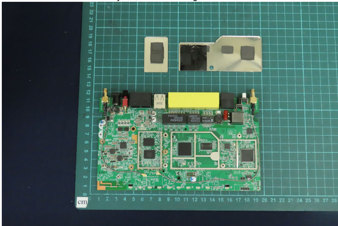
(41) EUT Photo - Brand Name: DrayTek, Model No.: Vigor2767Vax
