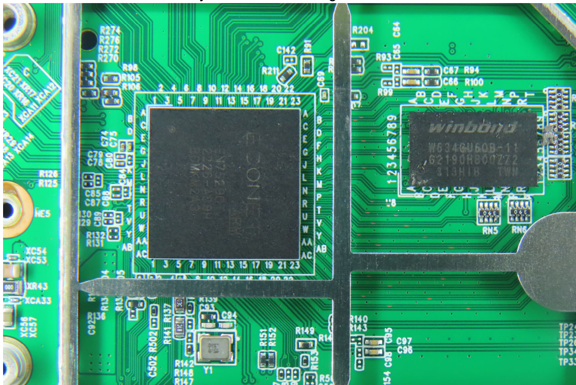
(44) EUT Photo - Brand Name: DrayTek, Model No.: Vigor2767Vax
