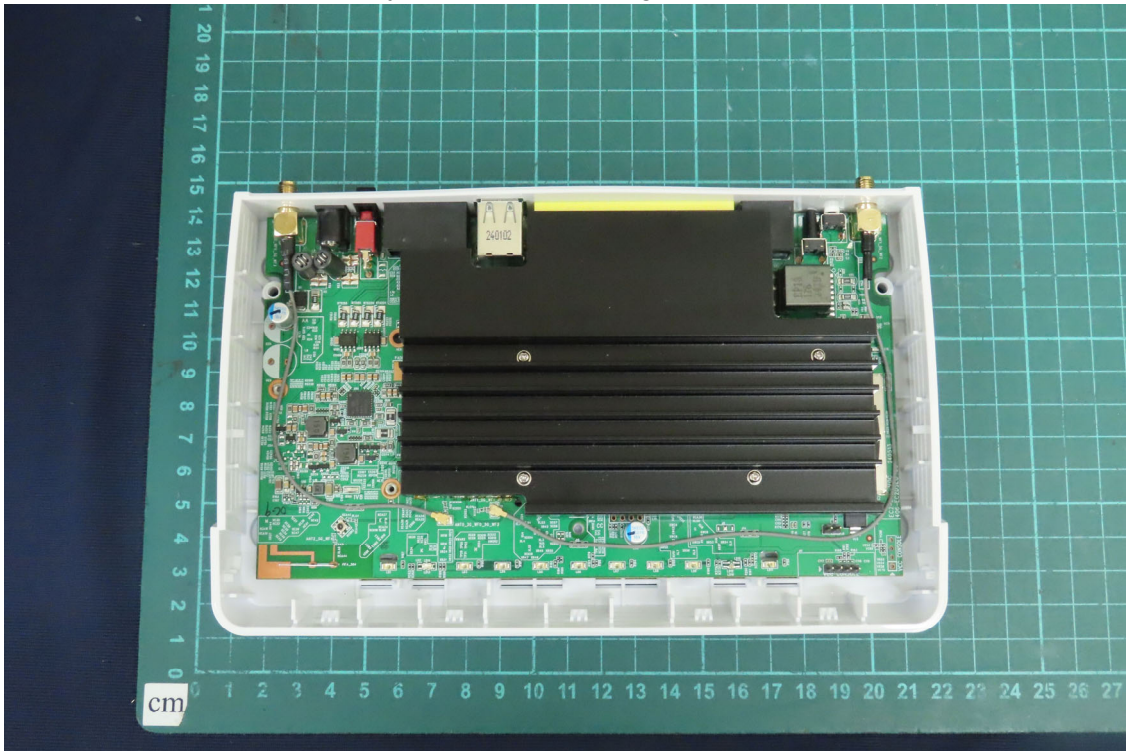
(36) EUT Photo - Brand Name: DrayTek, Model No.: Vigor2767Vax
