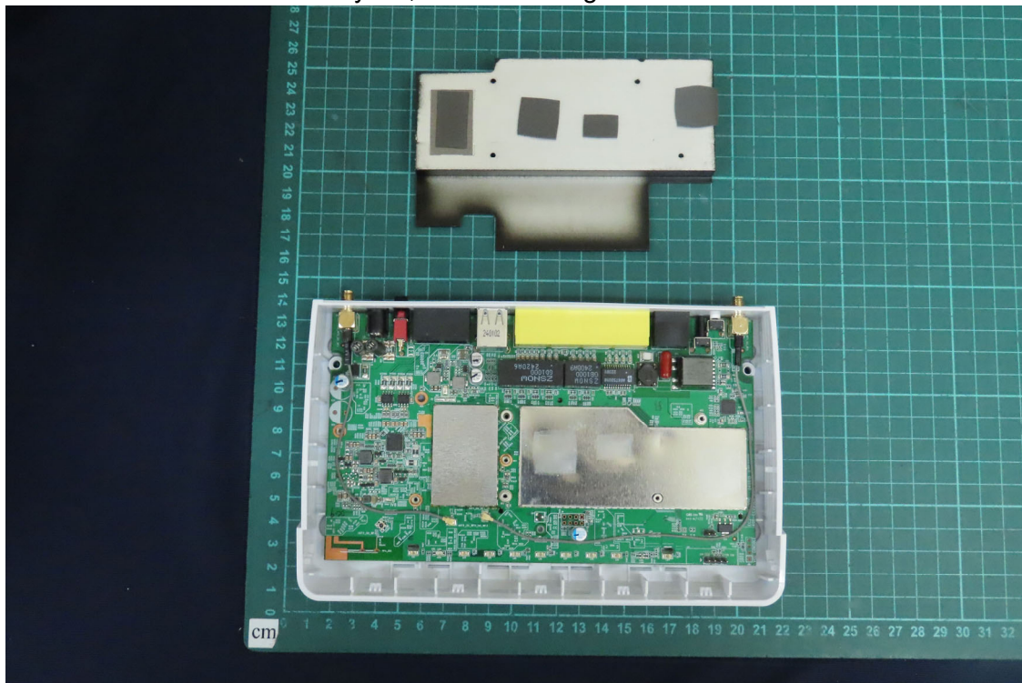
(37) EUT Photo - Brand Name: DrayTek, Model No.: Vigor2767Vax
