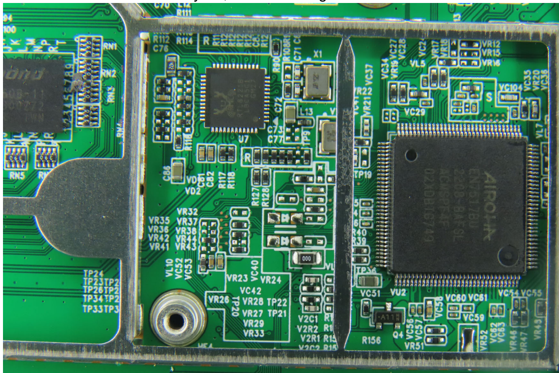
(43) EUT Photo - Brand Name: DrayTek, Model No.: Vigor2767Vax
