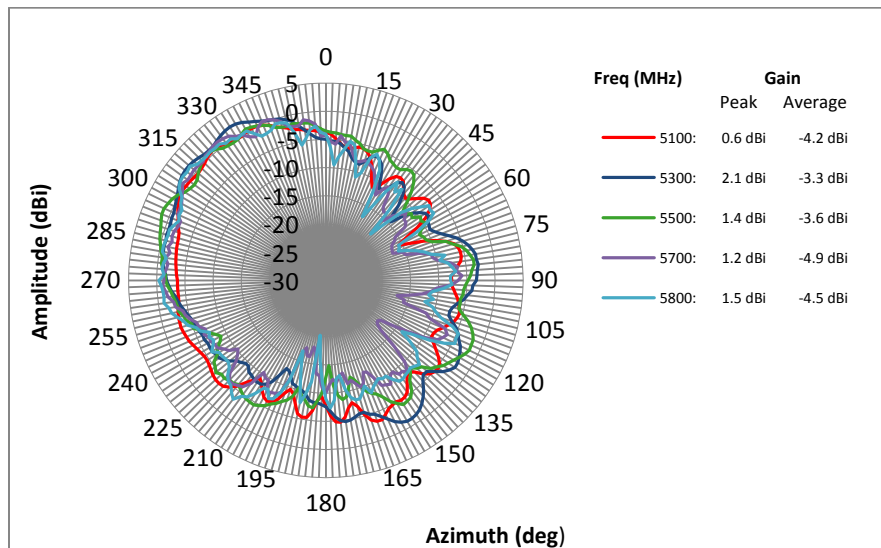
Typical H-plane radiation pattern @ 5 GHz
