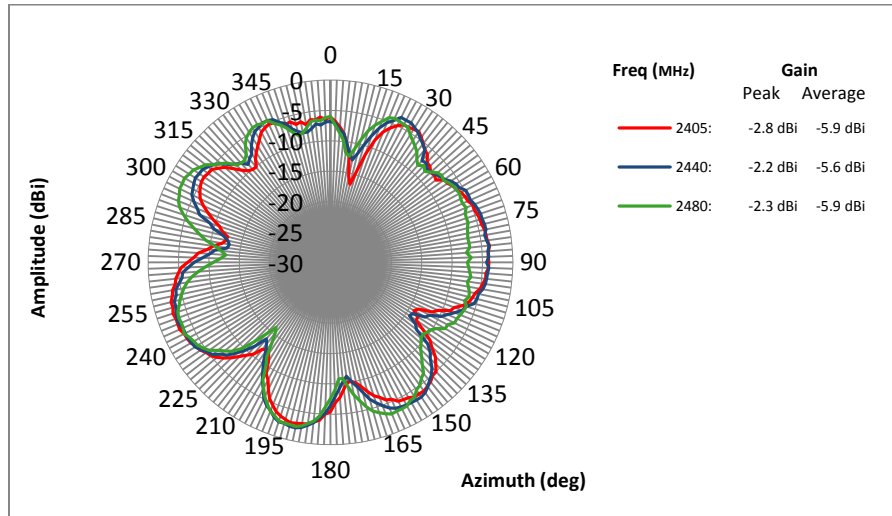
Typical H-plane radiation pattern @ 2.45 GHz
