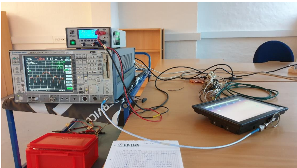
Photo 4. Frequency stability versus supply voltage and Occupied bandwidth test setup.
