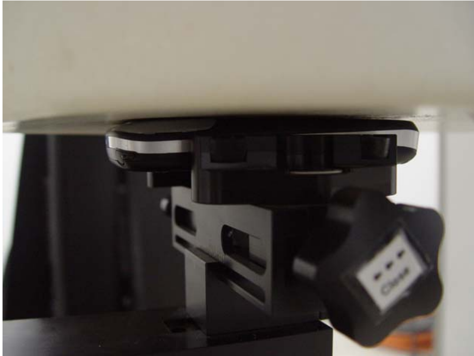
SAR Test Setup At Flat Phantom – Closer View (EUT Front Touched Phantom)
