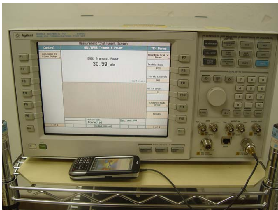
Conducted Power Measurement Setup – Far View
