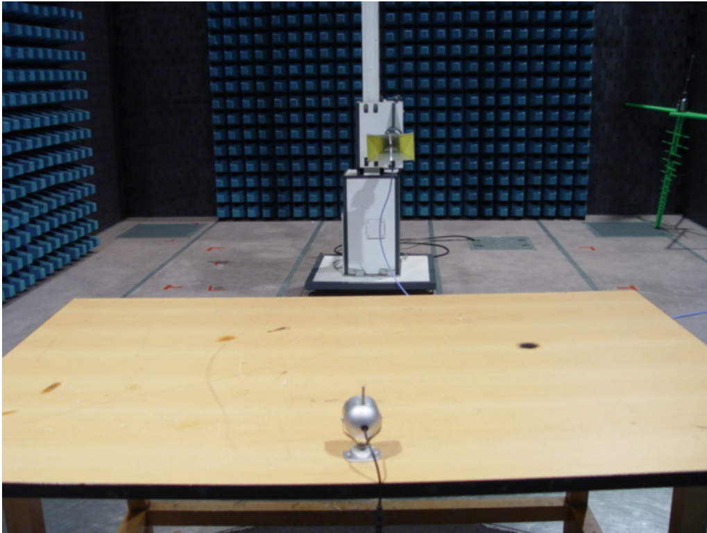
Photo 3 Radiated Emission Test
