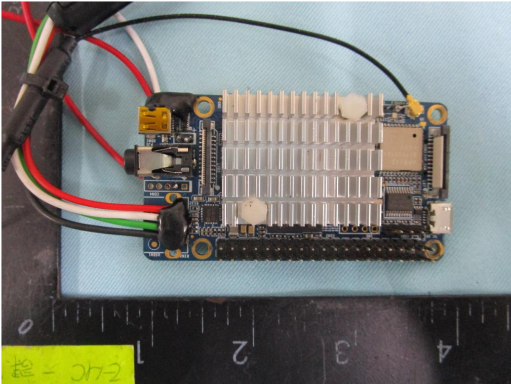
9. Front view of PCB 2
