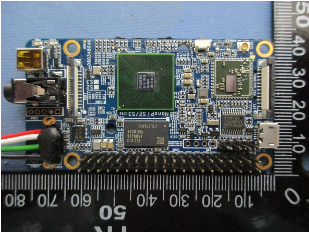
10. Front view of PCB 2 (Unshielded)
