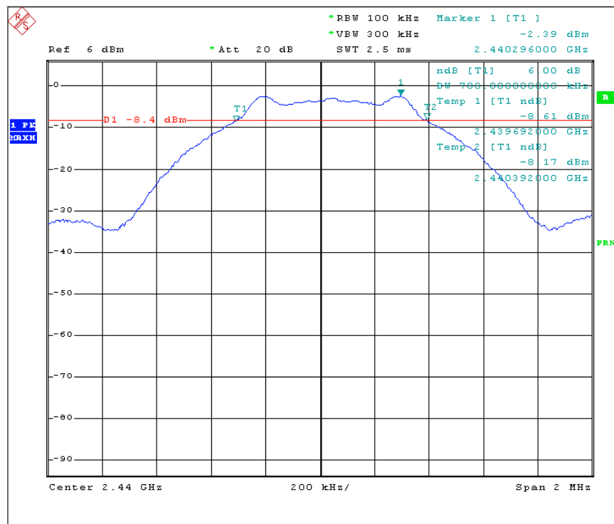
6dB Bandwidth, Middle Channel
