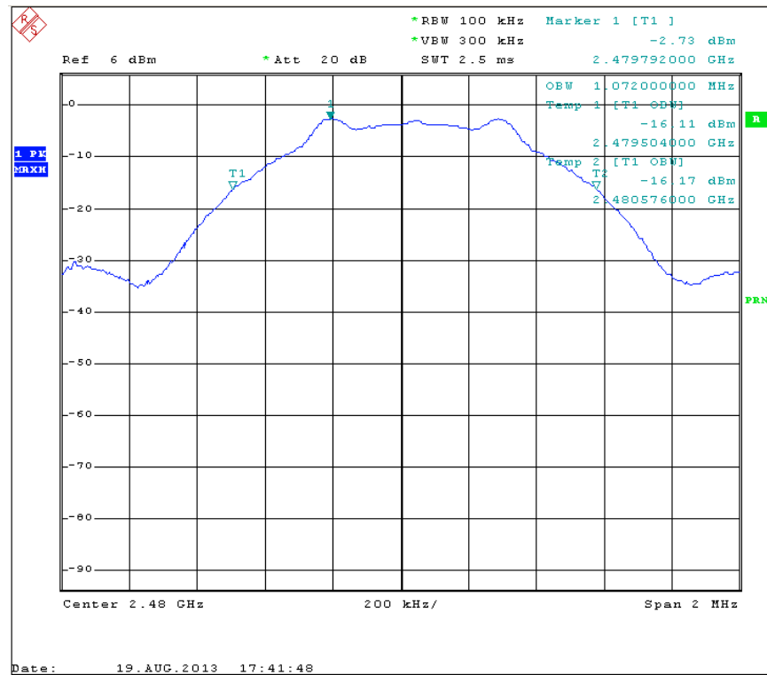
99% Bandwidth, High Channel
