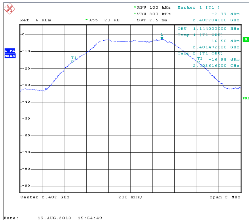
99% Bandwidth, Low Channel
