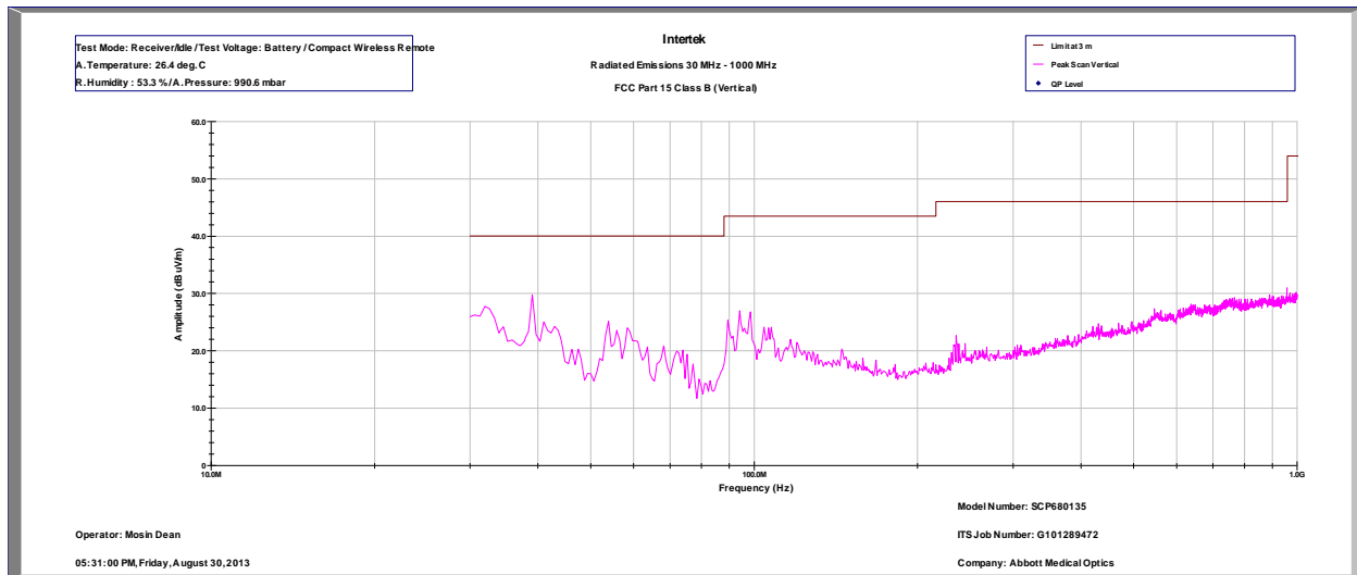
Radiated Emissions Peak Scan Vertical Polarization 30-1000 MHz for Compact Wireless Remote
