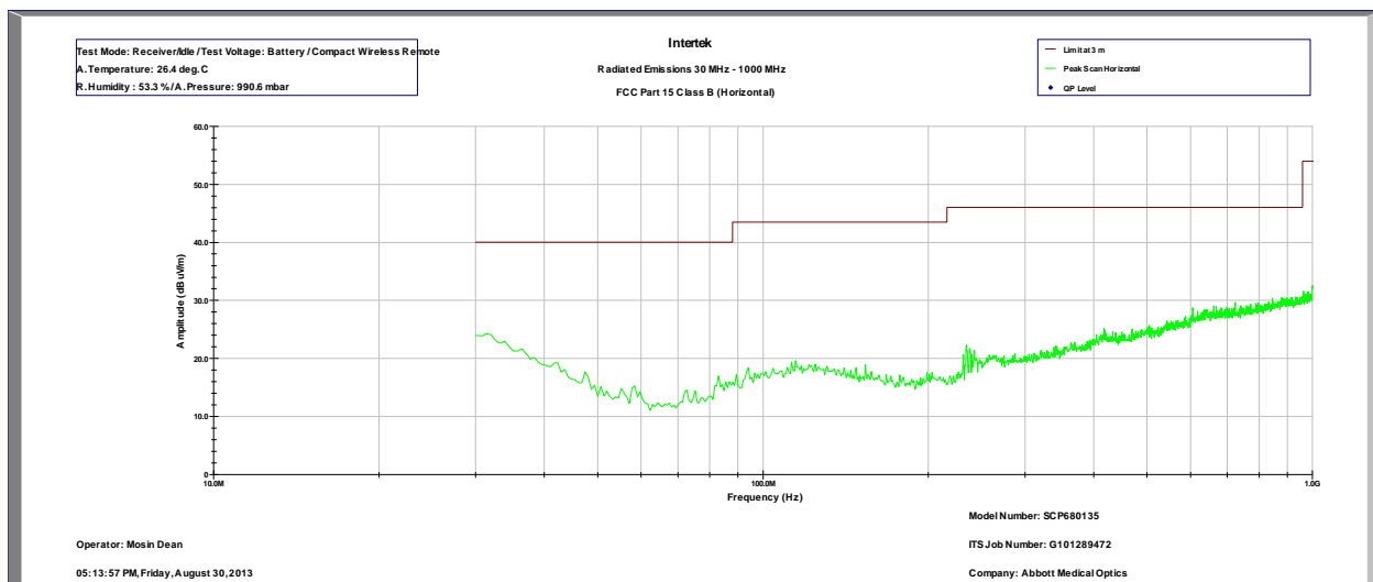
Radiated Emissions Peak Scan Horizontal Polarization 30-1000 MHz for Compact Wireless Remote
