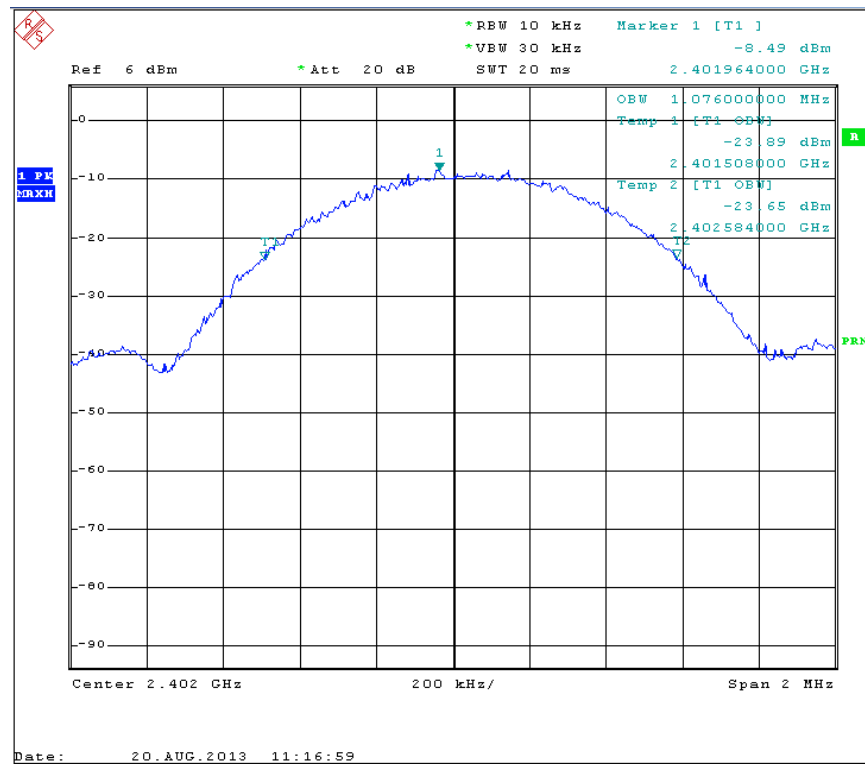
99% Bandwidth 10 kHz, Low Channel
