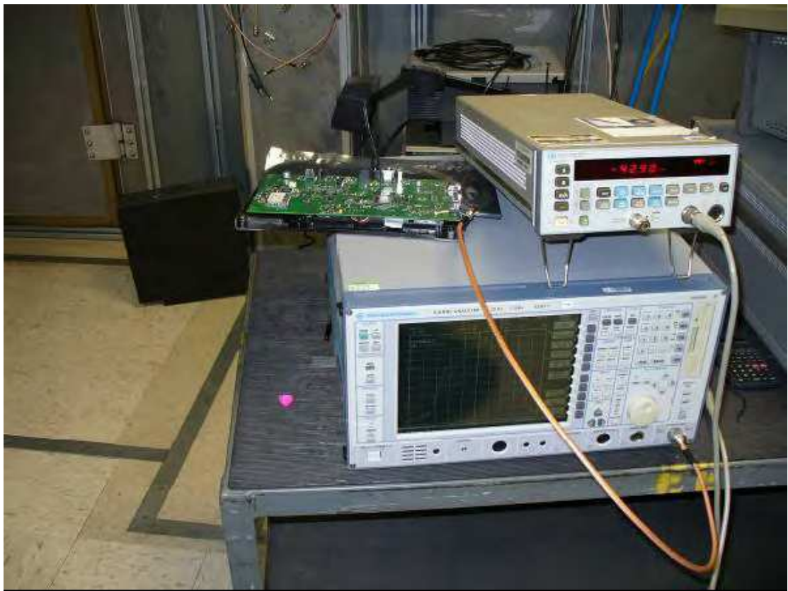
Conducted Power Setup
