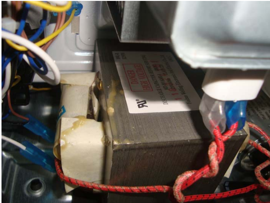
Transformer View
