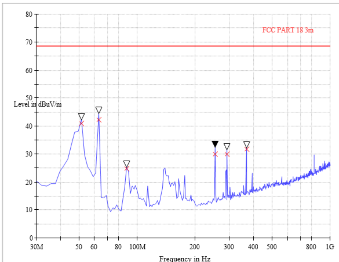
(Plot B: Test Antenna Vertical 30M - 1G)
