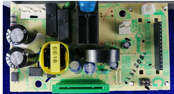
New Mother board –top view
