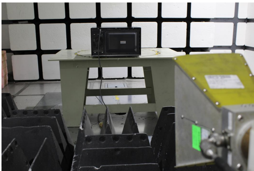
Radiated Emissions - Rear View (Above 1 GHz)
