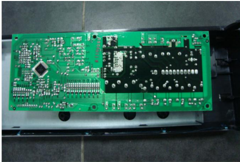
Mother board Bottom View
