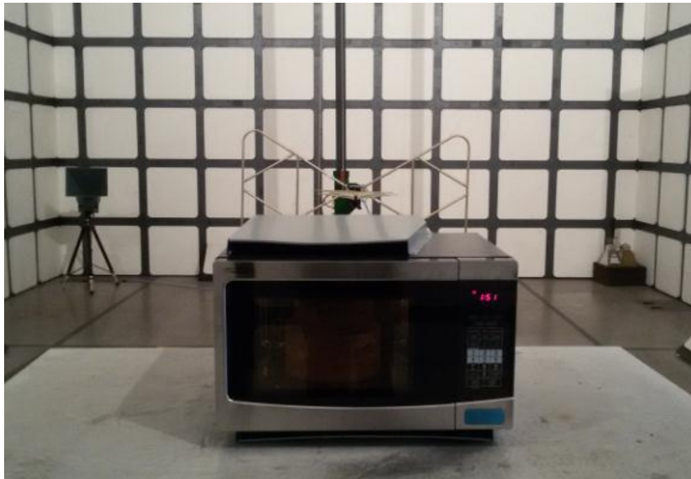
Radiated Emission Test Set-up (30 -1,000MHz):
