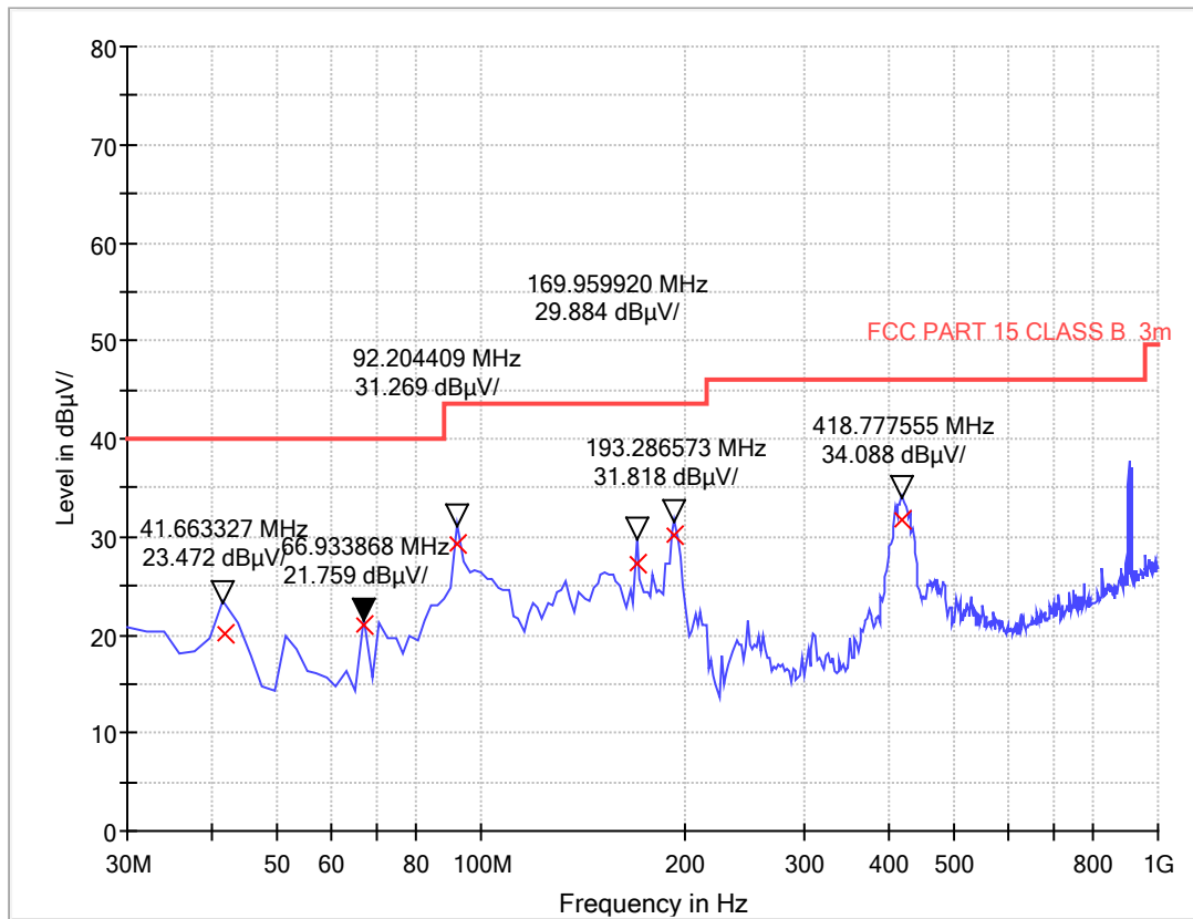
(Plot E: Test Antenna Horizontal 30M - 1G)
