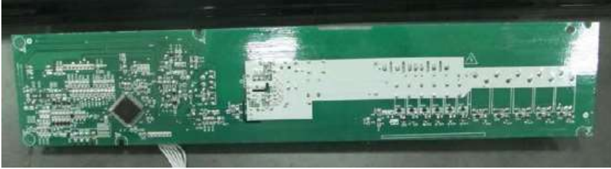
Original power board-bottom view
