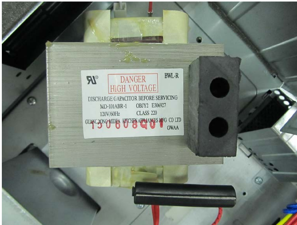
High-voltage Transformer View
