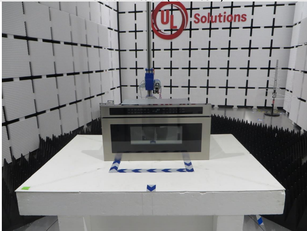
Radiated Emissions (1GHz~25GHz)
